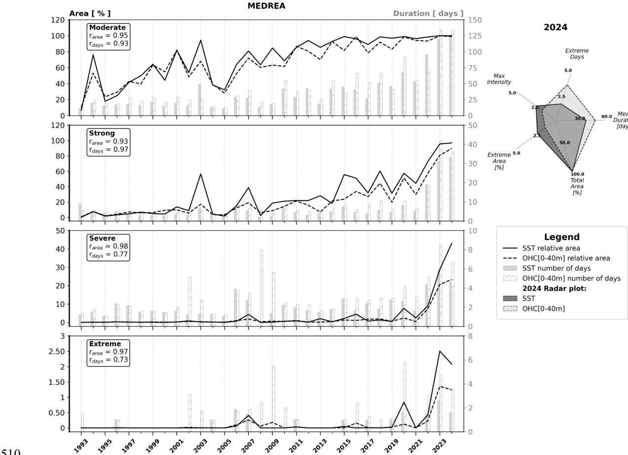
510 511 Figure 5: Time series of the temporal and basin-wide mean spatial coverage of MHW events in the Mediterranean Sea based on SST 512 (solid line) and OHC (dashed line) definitions. Results are derived from the Mediterranean Sea regional reanalysis (product ref. no. 513 4 in Table 1). The bars show the mean number of days of events for each category over the years, with SST-based values in grey and
