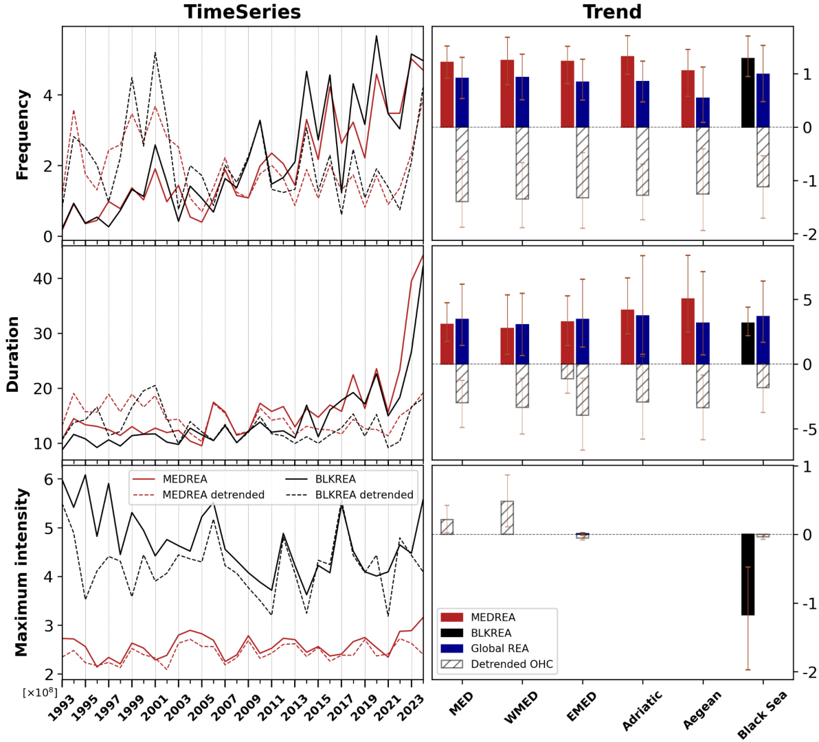
649 650 Figure A2: Left: time series of annual MHWs metrics number, duration (in days), and maximum intensity (in \text{J m}^{-2} ) – averaged over 651 the entire Mediterranean (red lines) and Black (black lines) Seas, comparing the OHC (0–40 m) definition without detrending (solid 652 lines) with the OHC-detrended approach (dashed lines), based on regional reanalysis data (product refs. no. 3 and 4 in Table 1). 653 Right: long-term trends (1993–2024) in MHWs number (events per decade), duration (days per decade), and maximum intensity 654 ( \text{W m}^{-2} ), derived from regional and global reanalyses (product ref. no. 3, 4 and 5 in Table 1), for selected (sub)regions following
