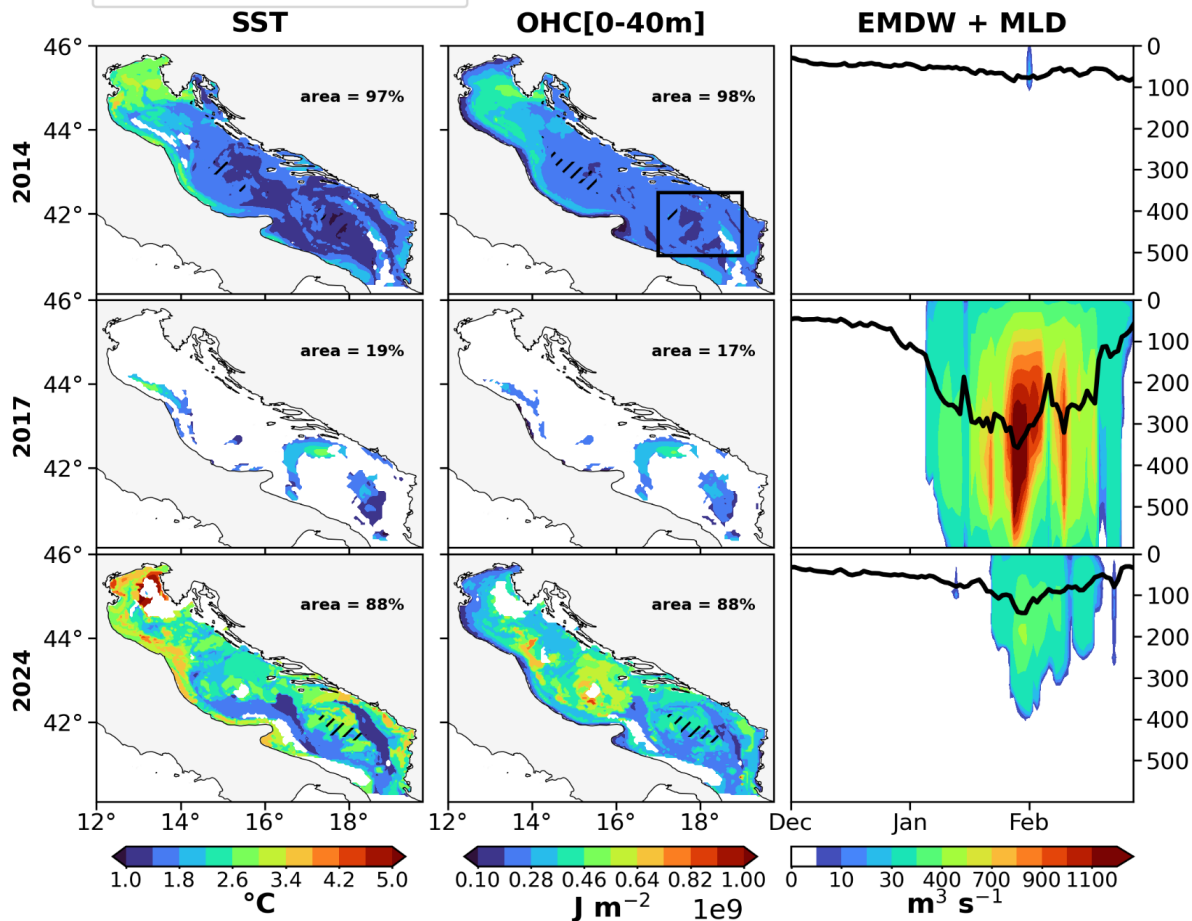
Figure 3: Upper plot: Time series show basin-averaged MHW frequency and duration (days) from two definitions based on SST and OHC, together with mean MLD during winter (1993–2024) in the SAP region. Lower plot: Spatial maps exhibit MHW maximum intensity based on SST ( ^{\circ}\text{C} ) on the left and OHC (0–40 m, \text{J m}^{-2} ) in the middle for 2014, 2017, and 2024 in the Adriatic Sea. The black rectangle on the 2014 OHC map indicates the SAP region. Hatched areas highlight regions where events lasted less than 10
