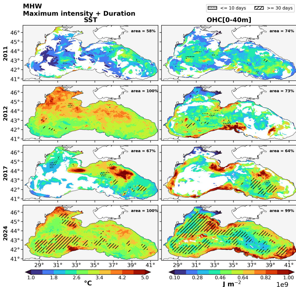
Figure 2: Spatial distribution of the yearly average of mean-maximum intensity of MHW events for selected years in the Black Sea using SST-based (left) and OHC-based (right) definition. Hatched areas highlight regions where events lasted less than 10 days or more than 30 days. Results are derived from the Black Sea regional reanalysis (product ref. no. 3 in Table 1).
