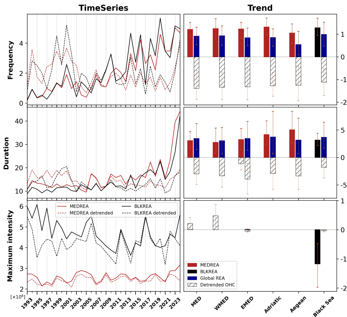
Figure A2: Left: time series of annual MHWs metrics number, duration (in days), and maximum intensity (in J m -2 ) – averaged over the entire Mediterranean (red lines) and Black (black lines) Seas, comparing the OHC (0–40 m) definition without detrending (solid lines) with the OHC-detrended approach (dashed lines), based on regional reanalysis data (product refs. no. 3 and 4 in Table 1). Right: long-term trends (1993–2024) in MHWs number (events per decade), duration (days per decade), and maximum intensity (W m -2 ), derived from regional and global reanalyses (product ref. no. 3, 4 and 5 in Table 1), for selected (sub)regions following Dayan et al. (2022). Brown lines indicate the 95% confidence interval. Solid bars show standard metrics definition, striped bars show SST de-trended metrics.
