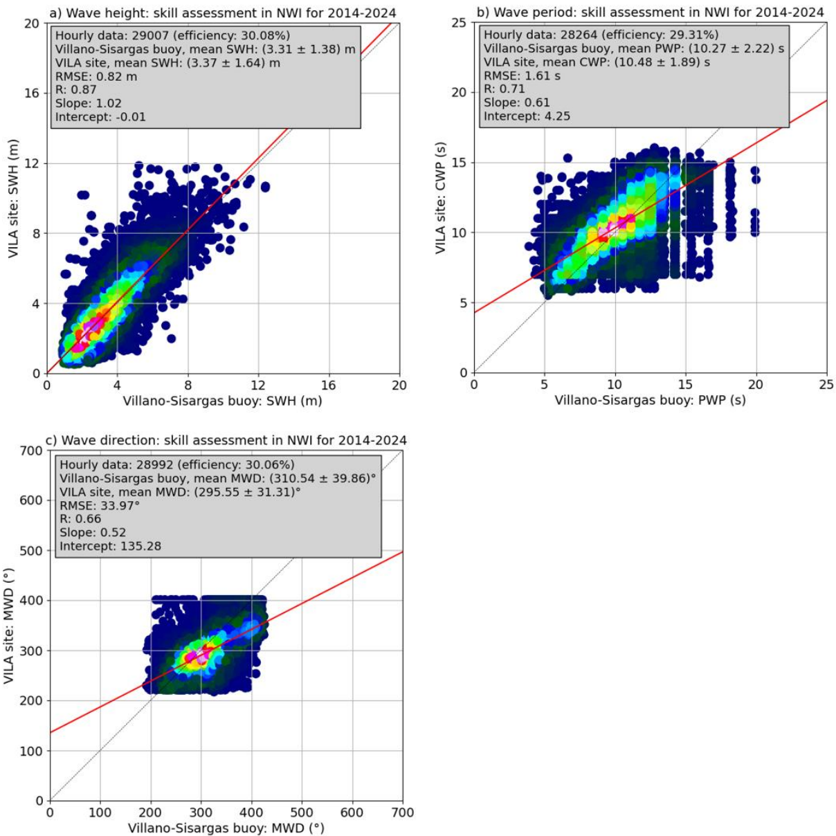
760 Figure A3. Long-term skill assessment of VILA site wave data at range cell 3 (RC3) -product ref. no. 4 in Table 1- against in situ observations provided by Villano-Sisargas deep-water buoy -product ref. no. 2 in Table 1- for the concurrent 11-year period (2014-2024): best linear fit (solid red line) of scatter plot between hourly observations of a) significant wave height (SWH), b) period (centroid and peak wave period -CWP and PWP, respectively-) and c) mean wave direction (MWD), where angles less than 60^\circ were adjusted by adding 360^\circ to improve visibility and facilitate 765 linear regression. The dotted black line represents the result of perfect agreement with slope 1.0 and intercept 0. Statistical metrics are presented in the grey box.
