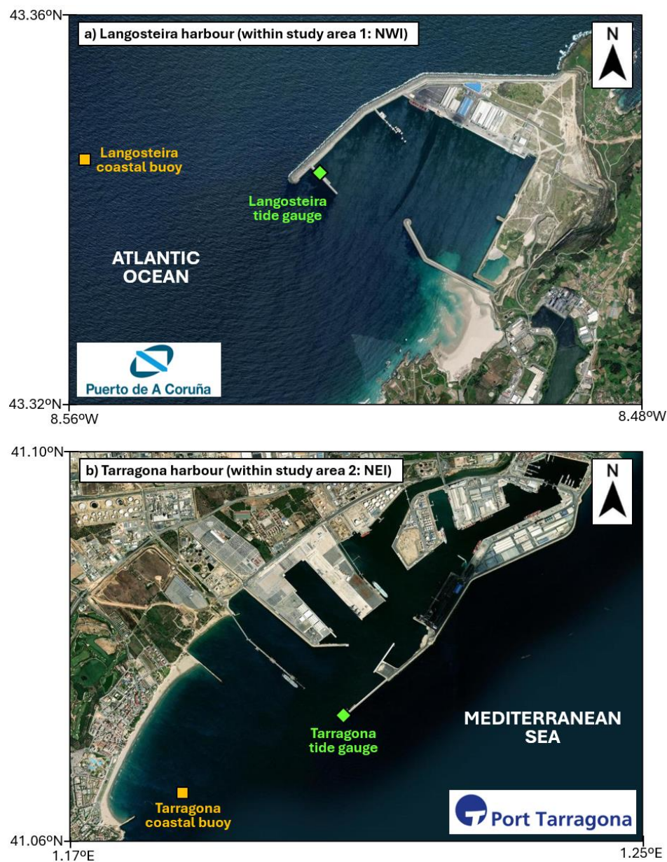
745 Figure A1. Aerial snapshot showing the geometry of two Spanish harbours: (a) Langosteira harbour (which belongs to A Coruña port authority), located in the northwestern Iberia (NWI) area and (b) Tarragona harbour, situated in the northeastern Iberia (NEI) area. Orange squares and green diamonds denote the location of coastal moored buoys and tide gauges, respectively. Map by © ArcgGis.
