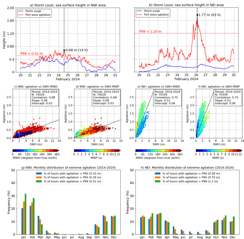
730 Figure 3. Hourly time series of storm surge (meteorological residual) and port wave agitation (product ref. no. 3 in Table 1) recorded during Storm Louis (20–29 February 2024) by (a) Langosteira and (b) Tarragona tide-gauges (Fig. 1A). The 99 th percentile (P99) thresholds for agitation are indicated by dashed red lines. Scatter plots relating port
