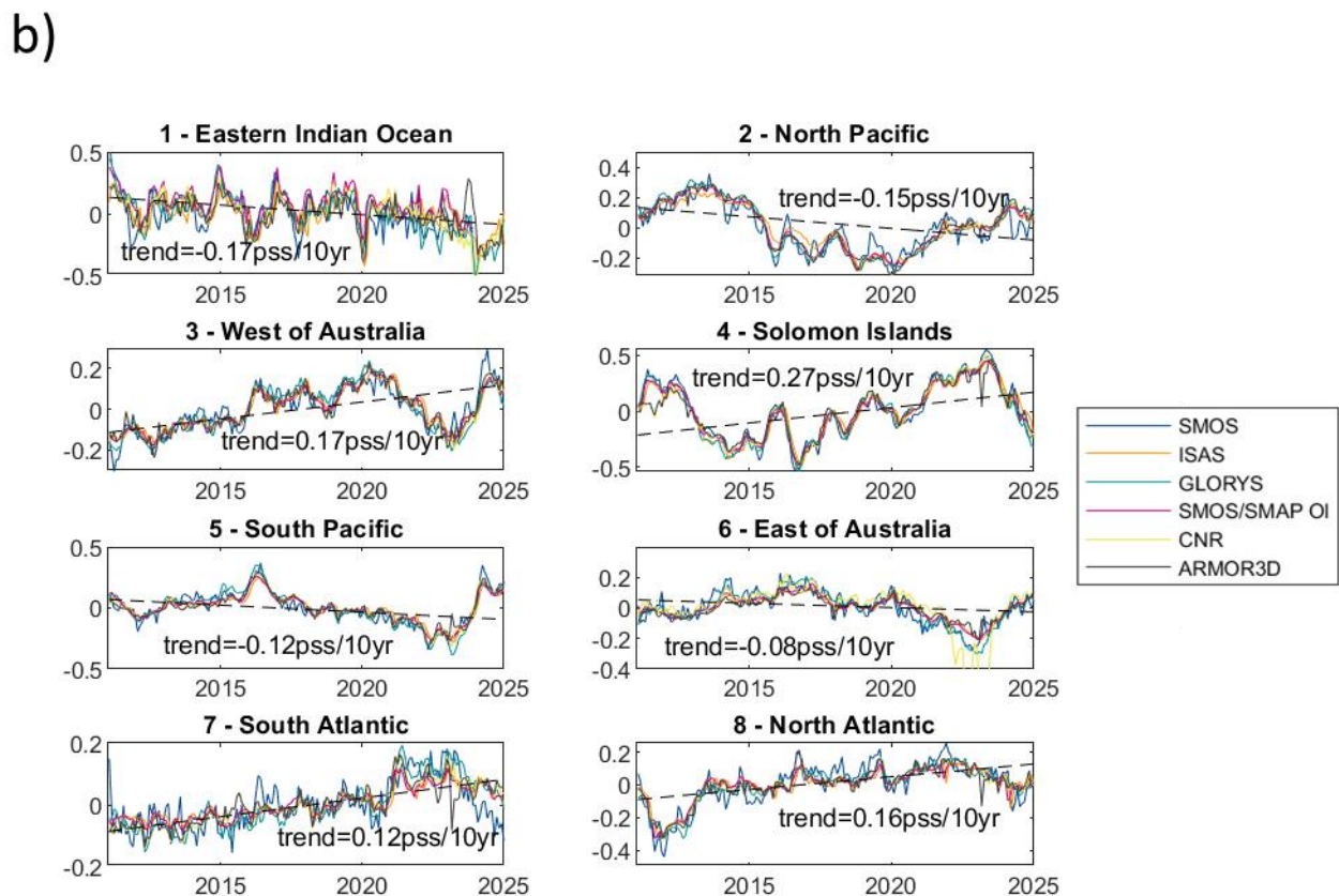
245 Figure 3: a) Regions selected to depict the mean SSS anomalies time series and their trends are defined by the red rectangles and correspond to the regions where the trends are significant in most of the products. Regions are ordered according to their mean SSS in the regions, from the freshest region (1) to the saltiest region (8). b) Time series of the SSS anomalies averaged over the regions selected in a): 1 is the Eastern Indian Ocean, 2 is the North Pacific, 3 corresponds to West of Australia, 4 to region of the Solomon Islands, 5 to South Pacific, 6 to South Atlantic and 8 to North Atlantic. The mean trend across all products for each region is 250 represented by the dashed line and indicated in each box.
