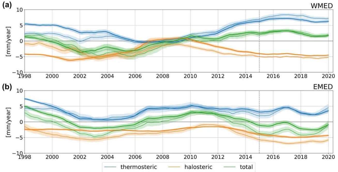
146 Figure 2: Time series of decadal trend associated to the de-seasoned total steric sea level ( \eta_s ), and its thermosteric ( \eta_t ) and halosteric 147 ( \eta_h ) components, computed over sliding windows shifted by one month across the period 1993–2024 in the WMED (a) and EMED 148 (b). Different datasets are shown: MEDREA24 (thick lines) and GLORYS12 (thin lines). Shaded areas represent the trend 149 uncertainty, defined as the standard deviation of the residuals from the bootstrap procedure. The vertical dashed line at Jan2015 150 marks the starting point of tide gauges analysis shown in Fig. 4.
