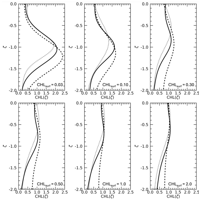
Figure A 2 – reconstructed vertical chlorophyll profiles from the Mediterranean model (solid lines), Morel and Berton (1989) (dashed lines) and Uitz et al. (2006) (dotted lines). The surface chlorophyll concentration (CHLsurf) is indicated in the bottom-right corner of each panel.
