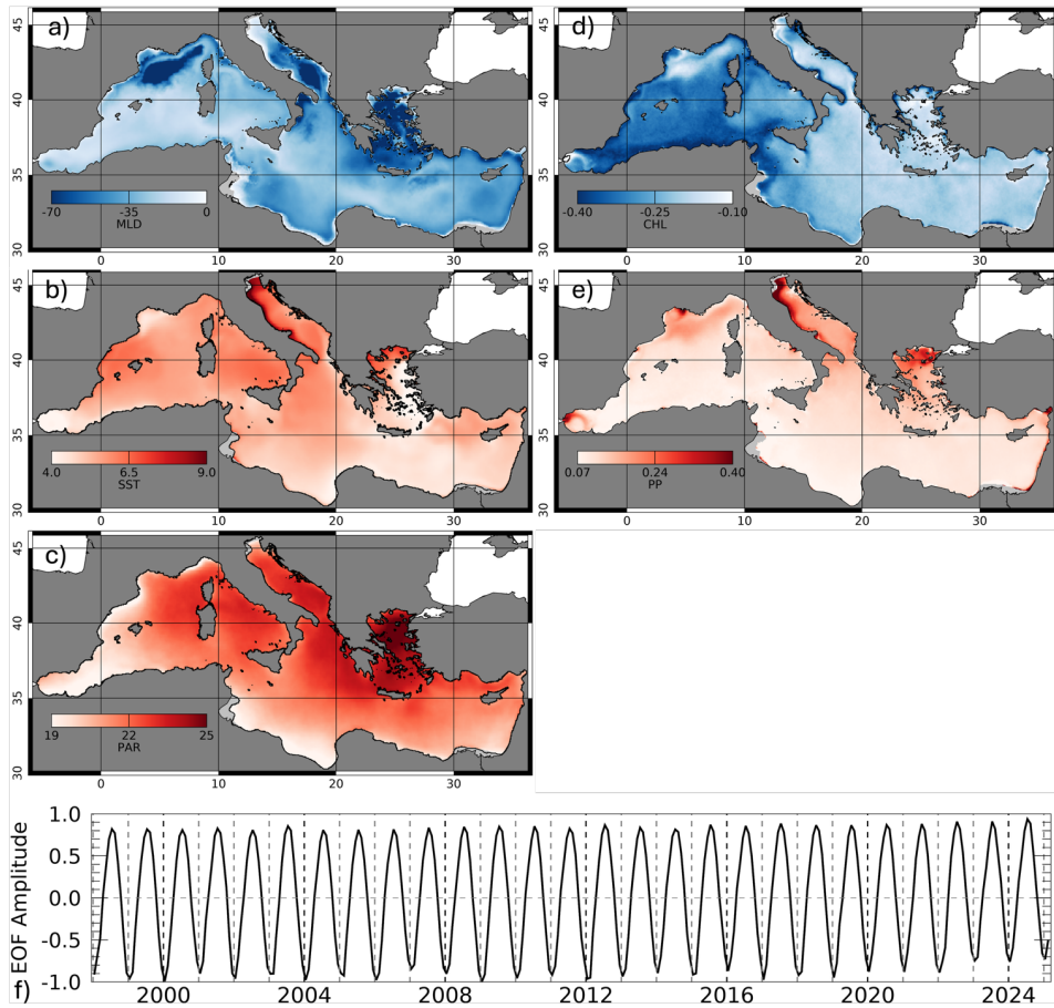
Figure 7 – First mode of MEOF of MLD (a), SST (b), PAR (c), CHL (d) and PP (e) spatial patterns and temporal evolution (f). Light grey indicates the areas permanently masked out because of persistent or recurrent Case II water conditions.
