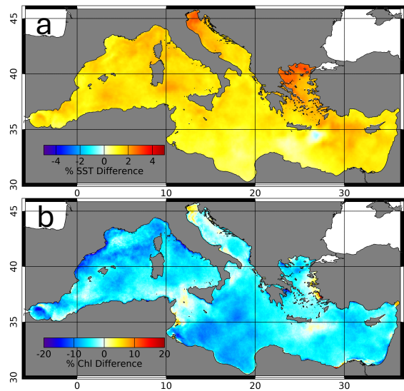
755 Figure B 1 – Relative percent difference RPD = 100 \frac{x-y}{y} , with Y being the mean time average (1998-2006) of SST and CHL for the same period as Volpe et al. (2012). X is the mean time average of SST (panel a) or CHL (panel b) computed over the full time range (1998-2025).
