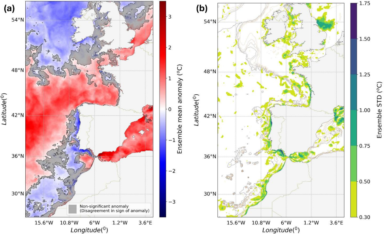
220 221 Figure 2: Results of the multi-product SST extremes indicator computed using the MULTI-OMI configuration. (a) Ensemble mean 222 of the 2024 anomaly of the 99th percentile of annual SST (blue/red shading) computed with respect to the reference period 1993- 223 2023. Grey shading indicates regions where at least one ensemble member shows an opposite sign of the SST anomaly, in which case 224 the anomaly sign is considered non-significant. (b) Standard deviation (STD) of the ensemble. Only STD values above 0.3 °C are 225 shown (contour shading), along with bathymetric contour lines at 50, 100, 500, 1000, 1500, 2000, and 3000 m depth (contour lines 226 over ocean areas).
