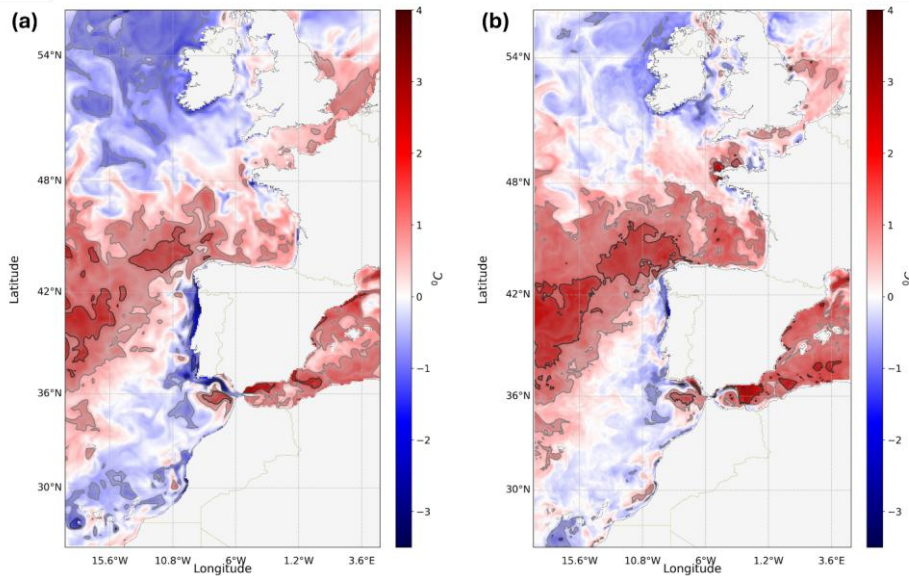
221 Figure 1: Anomaly in 2024 of the 99th percentile of the annual SST distribution (blue/red shading), referenced to the climatological 222 mean for the period 1993–2023 derived from the IBI reanalysis product (IBI-REA). Panel (a) shows results obtained using the OMI- 223 NRT configuration, which combines IBI-REA and the near real-time product IBI-NRT, while panel (b) displays results using the 224 OMI-INT configuration, which replaces IBI-NRT with the Interim dataset IBI-INT. Grey and black contour lines, along with partial 225 grey shading, indicate regions where the absolute anomaly exceeds one and two standard deviations, respectively, of the inter-annual 226 distribution of the 99th percentile during the reference period.
