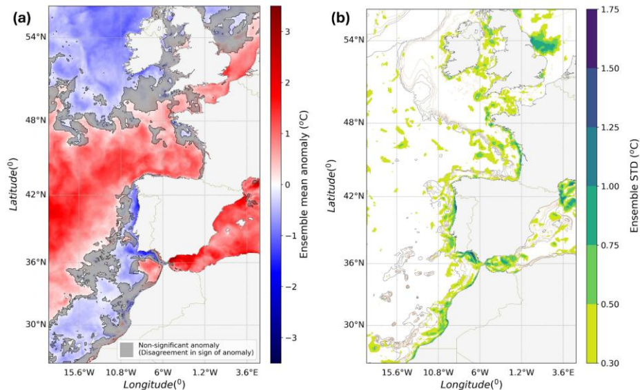
245 246 Figure 2: Results of the multi-product SST extremes indicator computed using the MULTI-OMI configuration. (a) Ensemble mean 247 of the 2024 anomaly of the 99th percentile of annual SST (blue/red shading) computed with respect to the reference period 1993-
