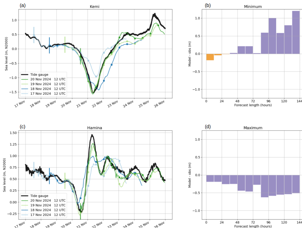
Figure 2: Analysis of BALMFC NRT forecast skill at Kemi (a,b) and at Hamina (c,d) during the Nov 2024 storm. In (a, c) the dark green, pale green, dark blue and pale blue lines show outputs from forecasts starting at noon on 20 Nov, 19 Nov, 18 Nov and 17 Nov respectively; these correspond to the 12-24 hour, 36-48 hour, 60-72 hour and 84-96 hour length forecasts assessed the time of the extreme sea levels. The first value in each forecast is indicated with a vertical line; each of the subsequent dots marks the end of a 12-hour period. The thick black lines in (a,c) show the time series of observations from each tide gauge. In (b, d) we show the difference between each forecast and the tide gauge observations in the sea level minimum (b, Kemi) and the sea level maximum (d, Hamina) as a function of forecast length, including all forecasts from the shortest (0-12 hours) to the longest (132-144 hours). Purple shading indicates that the model has underestimated the magnitude of the sea level extreme, orange shading indicates that the model has overestimated the magnitude of the sea level extreme.
