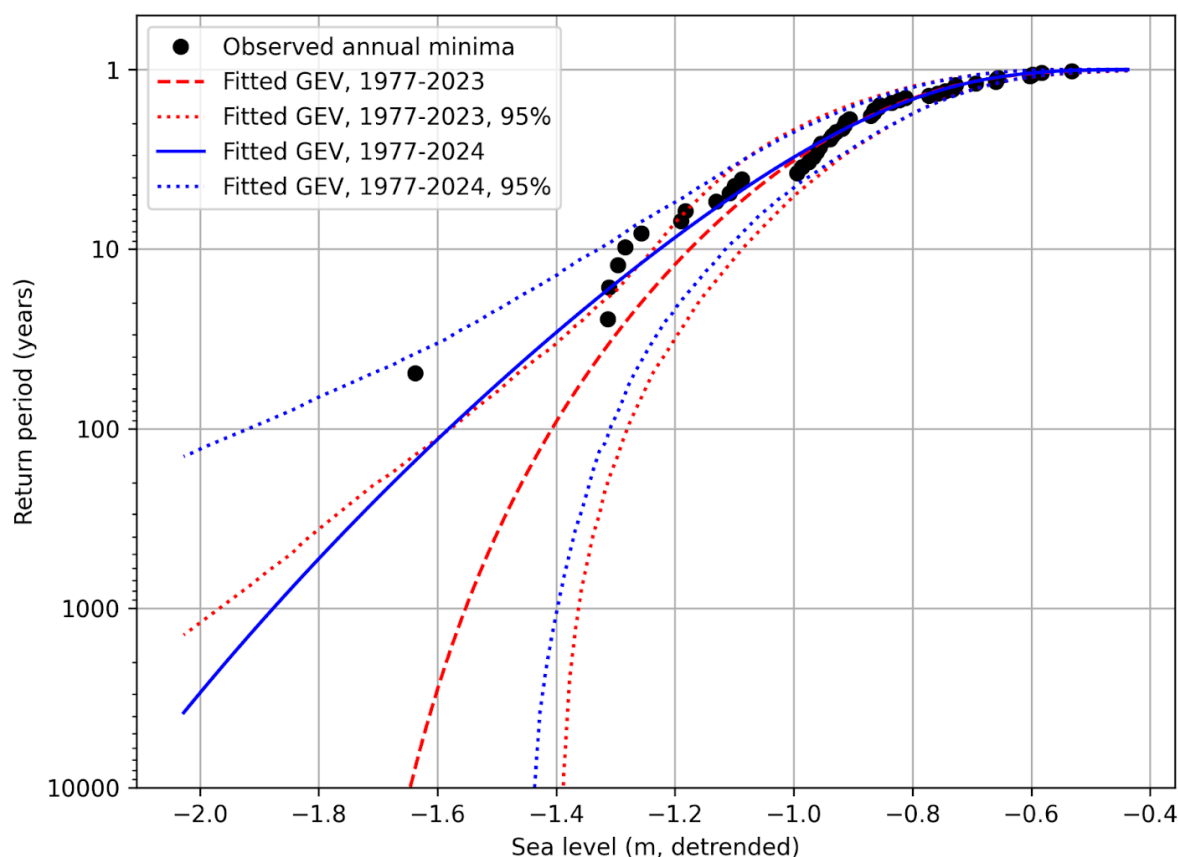
225 Figure 3. Cumulative probability distribution of Kemi annual minima 1977-2024. The observed minima in the N2000 height system were detrended by removing the trend of annual mean sea levels in 1977-2024, to exclude the effect of long-term mean sea level change. Generalized Extreme Value (GEV) distributions were fitted to the annual minima with the 2024 record value included in the fit (solid blue line), and without the 2024 value (dashed red line). The 95% confidence intervals (dotted lines) are based on 1000 nonparametric bootstrap samples.
