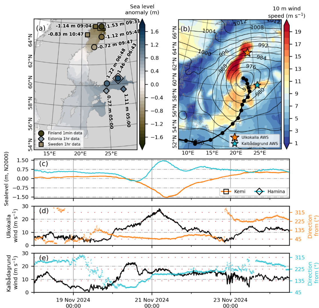
135 Figure 1: a) NEMO modelled sea level (shading) from the BAL-MFC NRT system, at 9:30 UTC on 21 Nov 2024, shown relative to the mean dynamic topography; overlaid with tide gauge data (from Finnish, Estonian or Swedish measurements as indicated on legend). Beginning at the westernmost station and following the coastline clockwise, the stations shown are Furuögrund, Kalix, Kemi, Raahe / Brahestad, Pietarsaari / Jakobstad, Helsinki, Hamina, Narva and Tallinn. Minimum measured sea levels on 21 Nov 2024 are shown in the Bothnian Bay, and maximum sea levels on 21 Nov 2024 are shown in the Gulf of Finland; in both cases the 140 timing of the minimum/maximum is displayed next to the measured sea level values in the RH2000/N2000/EH2000 reference system. Panel b) shows 10-metre wind speed (shading) and mean sea level pressure (contours) from the ERA5 reanalysis at 21 Nov 2024 06:00 UTC. The track of the storm from 6:00 UTC on 19 Nov 2024 to 6:00 UTC on 21 Nov 2024 is shown with the black line, with the location of the centre marked every three hours by a dot. Panel c) shows a time series of observed sea levels from Kemi 145 and Hamina (corresponding locations are marked with a square outline and a diamond outline respectively in panel a). Sea level values are shown in the N2000 height system with simultaneous wind measurements from Ulkokalla (d) and Kalbådgrund (e) AWS stations, locations marked in panel b).
