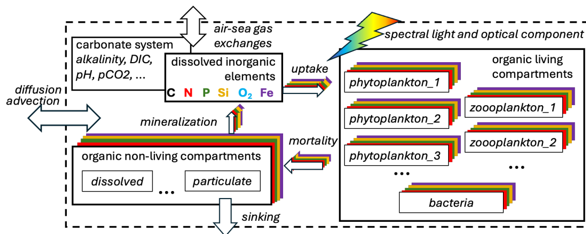
Fig. 1: simplified scheme of compartments (boxes) and processes (arrows) representing the cycles of multiple chemical elements typically included in a biogeochemical model. The symbol ... indicates the increase of the number of compartments and variable (e.g., multiple plankton functional types, multiple size compartments of non-living organic matter or additional variables resolved by the carbonate system).
