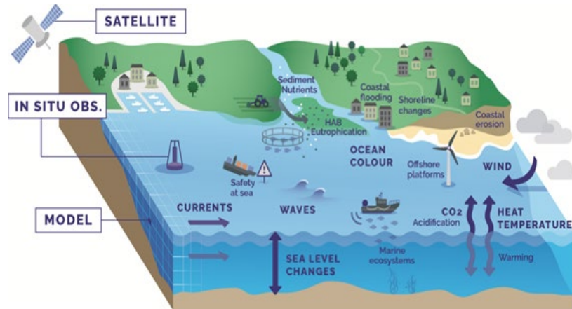
74 Figure 1: Schematic representation of the coastal zone, hazards (e.g. HAB (harmful algae bloom), metocean and biogeochemical 75 variables, as well as observations and applications (adapted from Melet et al., 2020).
