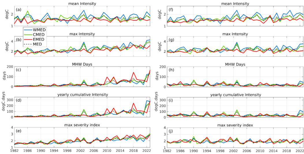
Figure 2: Temporal evolution and linear trends of MHW characteristics over 1982-2023 using the non-detrended (a-e) and the detrended SST anomaly timeseries (f-j). From top to bottom: Mean intensity (a,f), maximum intensity (g,b), Number of MHW days (c,h), yearly cumulative intensity (d,i), and maximum severity index (e,j). Blue, green and red lines and the black dashed line correspond to spatial averages for the western (WMED), central (CMED), eastern (EMED) Mediterranean sub-basins and the entire Mediterranean basin (MED), respectively. The WMED, CMED and EMED sub-regions are separated by the strait of Sicily, and a fixed longitude boundary at 22° E. Product used: Mediterranean Sea High Resolution L4 Sea Surface Temperature Reprocessed (Table 1, product ref. no.1).
