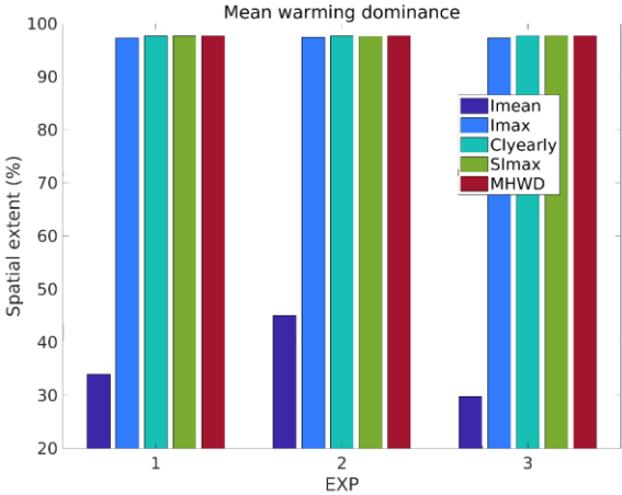
310 Figure 4: Sensitivity of the Trend Attribution Ratio (TAR) to different approaches for base climatology used in MHW detection in the original (non-detrended) dataset. Vertical axis: Percentage of Mediterranean locations with positive TAR (i.e., mean warming dominance in trends of MHW metrics). Horizontal axis: (EXP 1) Climatology computed based on the detrended dataset with reference period 1982–2023; (EXP 2) Climatology computed based on the non-detrended dataset with reference period 1982– 2023; (EXP 3) as EXP 2 but with reference period 1982–2002. Metrics used: Mean intensity (I mean ), maximum intensity (I max ), 315 Number of MHW days (MHWd), yearly cumulative intensity (C Iyearly ), and maximum severity index (S Imax ). Product used: Mediterranean Sea High Resolution L4 Sea Surface Temperature Reprocessed (Table 1, product ref. no.1).
