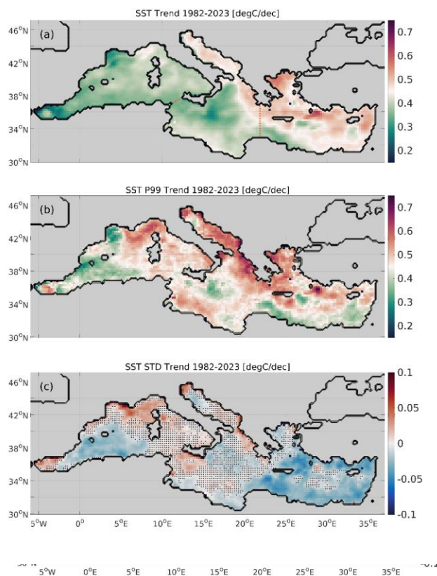
Figure 1: Linear trend of (a) SST, (b) the 99 th percentile (P99) of SST and (c) the standard deviation (STD) of SST, for the period 1982-2023, using de-seasonalized SST anomalies. Black dots superimposed on trend fields denote the locations with statistically insignificant trends (Mann Kendall test, 95% confidence level). The western, central and eastern sub-basins are separated by the strait of Sicily, and a fixed-longitude boundary at 22° E, respectively (red dashed lines in (a)). Product used: Mediterranean Sea High Resolution L4 Sea Surface Temperature Reprocessed (Table 1, product ref. no.1).
