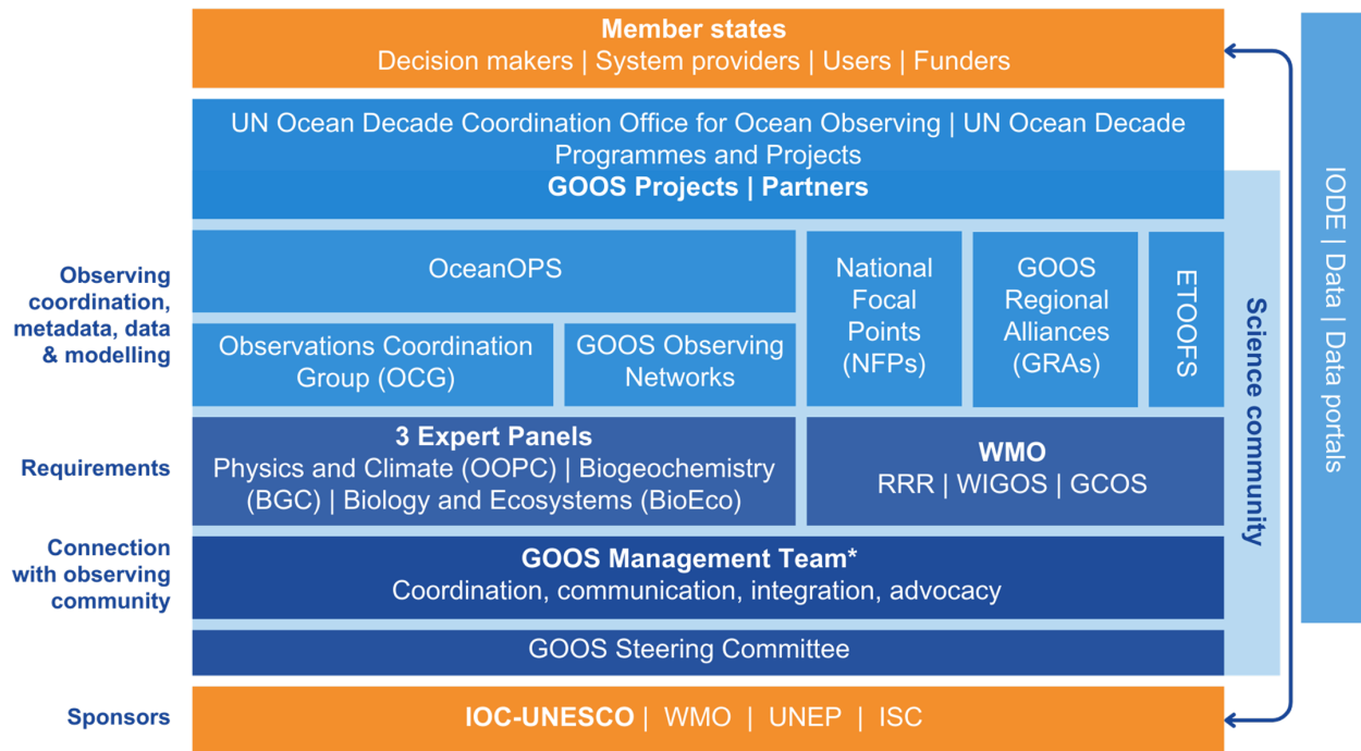
Figure 1: GOOS framework
