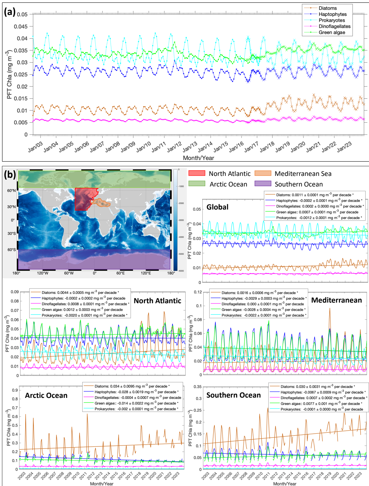
Figure 4. Panel (a): Updated (corrected) time series of the five PFT Chl a based on the global mean from 2002 to 2023. Merged sensor-derived PFT products cover the period of July 2002–April 2017 (indicated with dots), and OLCI-derived PFT products are for May 2016–Dec 2023 (indicated with crosses). Note that the OLCI-derived products have been corrected to merged products based on MLBE. Panel (b): Trends of diatoms, haptophytes, dinoflagellates, green algae and prokaryotes Chl a on the global scale and four regional scales (the North Atlantic Ocean, the Mediterranean Sea, the Arctic Ocean and the Southern Ocean), respectively. Trend slopes per decade with uncertainties have been indicated with significant trends marked with an asterisk (*).
