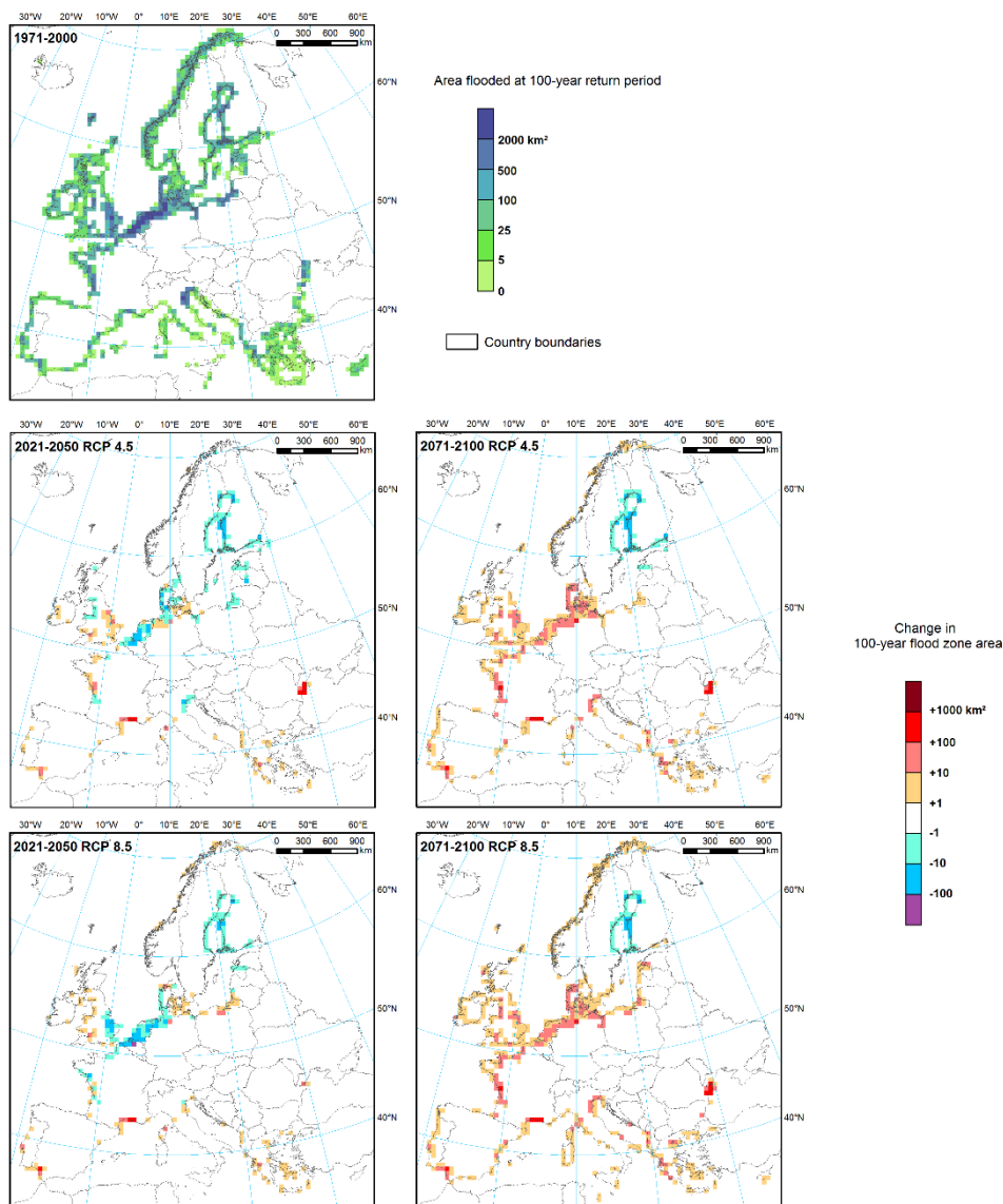
395 Figure 6: Indication of the current area vulnerable for flooding with a return period of once in a hundred years and for two different time slices under two different climate scenarios. From Paprotny et al. (2018).
