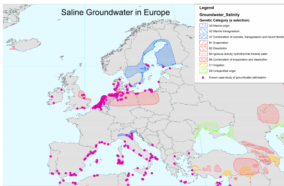
700 Figure 12: Case-studies where groundwater salinisation is occurring in the coastal zone around Europe (updated and after Post et al., 2018, and Van Weert et al., 2009), where it may cause multifaceted impacts combined with sea-level rise changes.
