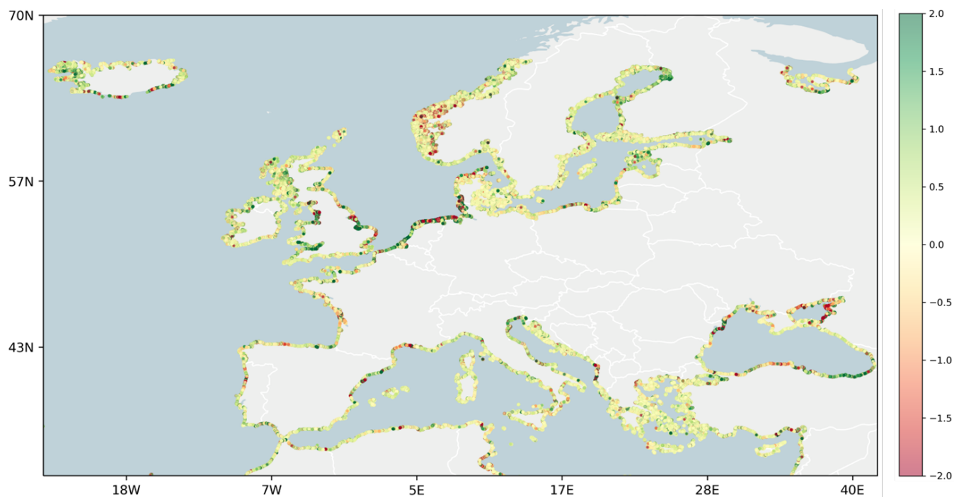
Figure 8: Long-term shoreline changes of the European beaches in m/yr since 1984. The red and green points indicate erosion and accretion respectively (data based on Luijendijk et al. (2018)).
