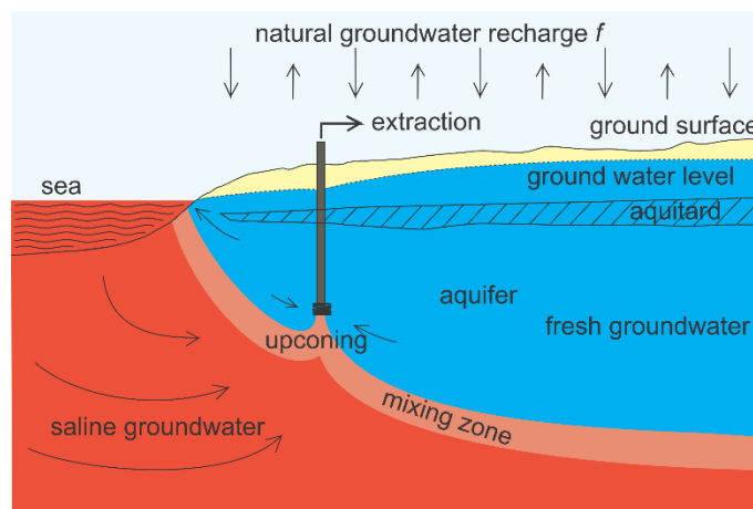
770 Figure 14: Saltwater intrusion in a coastal aquifer where too much groundwater is extracted leading to upconing of saline groundwater into the extraction well.
