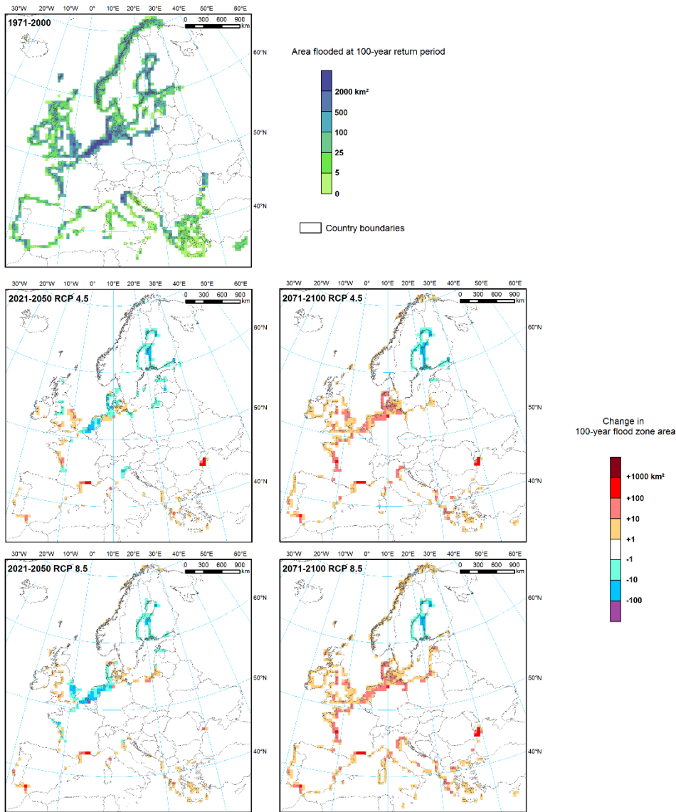
405 Figure 6: Indication of the current area vulnerable for flooding with a return period of once in a hundred years and for two different time slices under two different climate scenarios. From Paprotny et al. (2018).
