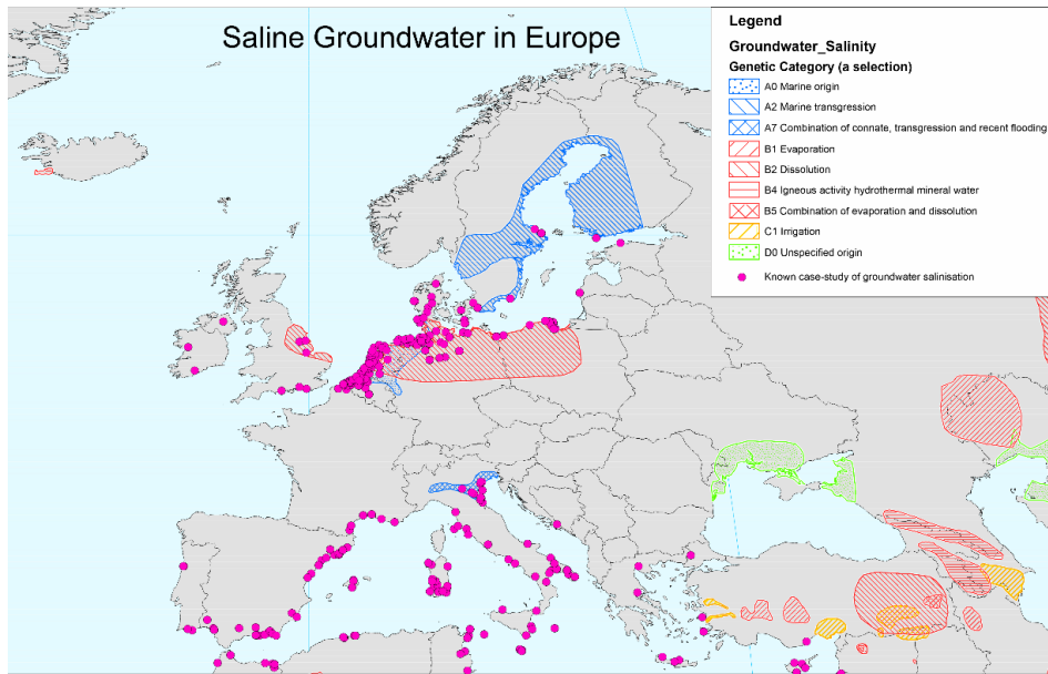
720 Figure 12: Case-studies (not exhaustive) where groundwater salinisation is occurring in the coastal zone around Europe (updated and after Post et al., 2018 and Van Weert et al., 2009), where it may cause multifaceted impacts combined with sea-level rise changes.
