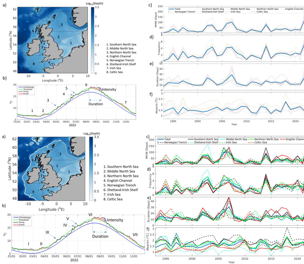
Figure 1: a) Map of North West European Shelf Sea with sub-region division (data from Table 1 ref. 1). Dashed curve indicates 200 m isobath. b) Detection of MHW events and their characteristics in 2022 (data from Table 1 ref. 1 & 2) near the Dogger Bank region in the southern North Sea (region 1 in panel a); c-f) Variations of MHW characteristics between 1993 and 2022, with the bold solid curve indicating the mean of total subdomains of the NWES (daily SST data from Table 1 ref. 1 & 2).
