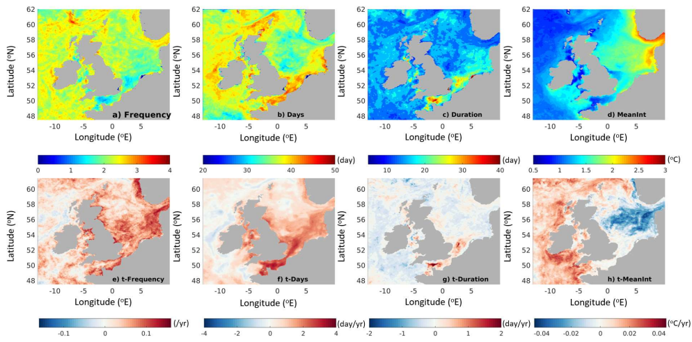
Figure 2. Mean and trend of MHW in the past 30 years (1993-2022). Dashed lines indicate 200 m isobath. (daily SST data from Table 1 ref. 1 & 2).
