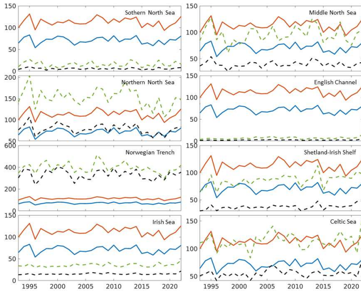
Figure 3. Potential energy anomaly ( \alpha , \text{J m}^{-3} ) between 1993 and 2022. The solid curves denote the spatial mean PEA of the entire NWES domain. The red curves represent the summer period (June-September, July-August) mean (in red solid) and the blue curves for the annual mean (blue solid) over the spatial mean of the entire NWES domain, respectively. The spatial mean PEA of different subdomains of the NWES (see Figure 1a) is indicated by dashed curves, with the green and black dashed curves are similar as the red and blue curves, but for different subdomains the annual mean and summer mean, respectively. (see Figure 1a).
