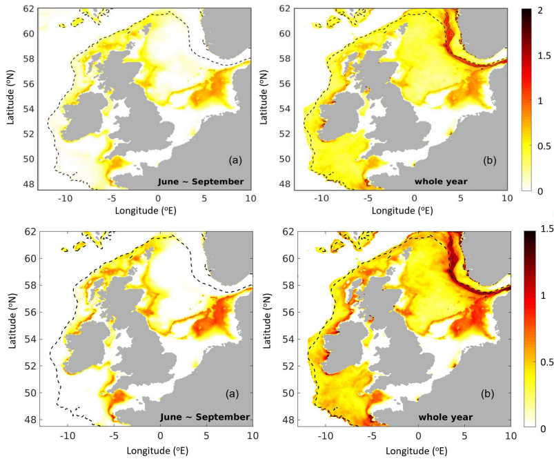
Figure 5. Ratio of the number of water stratification days to the number of MHW days for (a) June to September (summer period) and the whole year. The ratio is computed with Eq.4 using multi-year water temperature, salinity at different depths for 1992 to 2022 (Details are in Table 1 ref 1-&2). The thin dashed line indicates the 200 m isobaths.
