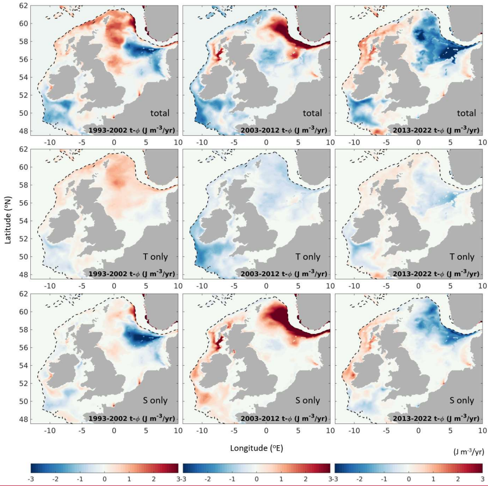
470 Figure 4. Trend of potential energy anomaly ( \phi , \text{J m}^{-3} \text{yr}^{-1} ) in the last 30 years. The first row (total) shows \phi computed with eq. 1, where density depends on both temperature (T) and salinity (S) in the water column. The second and third row are similar as the first row but with density depends only on either T or S, respectively.
