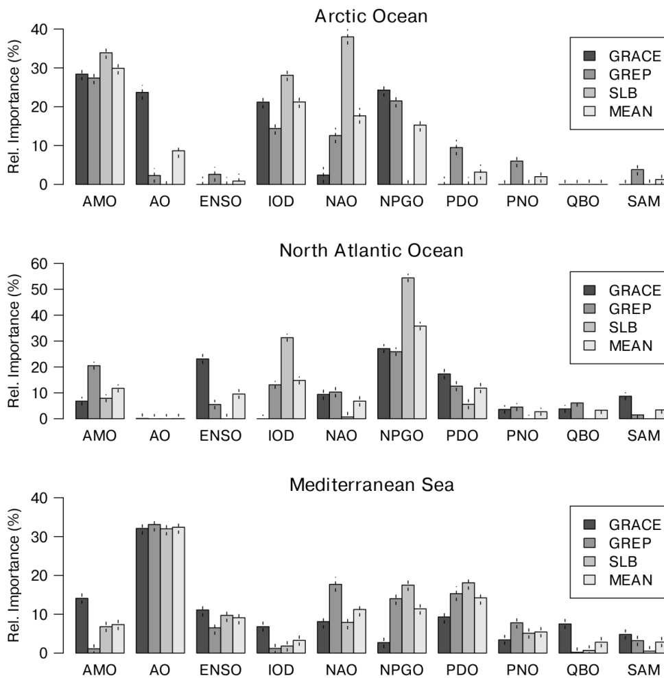
615 Figure 3. Relative importance (defined in the text in section 2.4) of the selected climate indices for the manometric sea level in the three basins investigated in this study, using the three datasets GRACE, GREP, and SLB. Also shown is the mean of the relative importance over the three datasets (indicated as MEAN). The climate indices acronyms are as follows: AMO: Atlantic Multidecadal Oscillation; AO: Arctic Oscillation; ENSO: multivariate El Niño Southern Oscillation; IOD: Indian Ocean Dipole; NAO: North Atlantic Oscillation; NPGO: North Pacific Gyre Oscillation; PDO: Pacific Decadal Oscillation; PNO: Pacific North American Oscillation; QBO: Quasi-Biennial Oscillation; SAM: 620 Southern Annular Mode. Vertical bars indicate the regression coefficients' standard errors.
