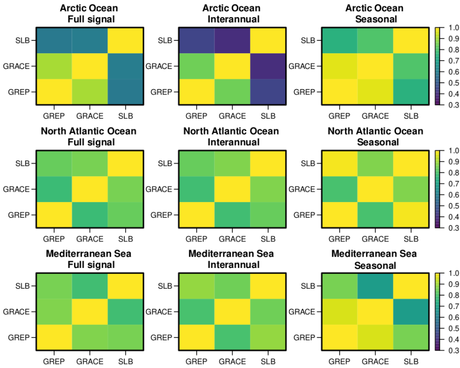
Figure 2. Correlation matrix for the three datasets in the three ocean basins investigated in this study, for both the full, the interannual, and the seasonal signals. All values of correlation are statistically significant, at the 99% confidence level. Note that the correlation matrix is symmetric, but all terms are shown in any case for the sake of clarity; note also that the minimum correlation in the palette is 0.3, whereas as the minimum correlation across all data shown is 0.39.
