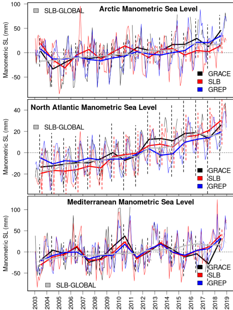
595 Figure 1. Manometric sea level timeseries for the Arctic, Mediterranean, and North Atlantic basins. Both monthly (thin lines) and yearly (thick lines) means are shown for GRACE, SLB, and GREP. The global barystatic sea level (SLB method) is also added in gray. The North Atlantic Ocean is defined from 0°N to 67°N, and the Arctic Ocean from 67°N
