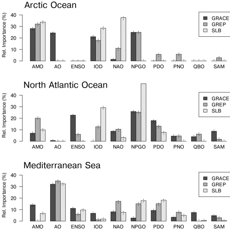
600 Figure 3. Relative importance (defined in the text in section 2.4) of the selected climate indices for the manometric sea level in the three basins investigated in this study, using the three datasets GRACE, GREP, and SLB. The climate indices acronyms are as follows: AMO: Atlantic Multidecadal Oscillation; AO: Arctic Oscillation; ENSO: multivariate El Niño Southern Oscillation; IOD: Indian Ocean Dipole; NAO: North Atlantic Oscillation; NPGO: North Pacific Gyre Oscillation; PDO: Pacific Decadal Oscillation; PNO: Pacific North American Oscillation; QBO: Quasi-Biennial Oscillation; SAM: Southern Annular Mode. Vertical bars indicate the regression coefficients' standard errors. 605
