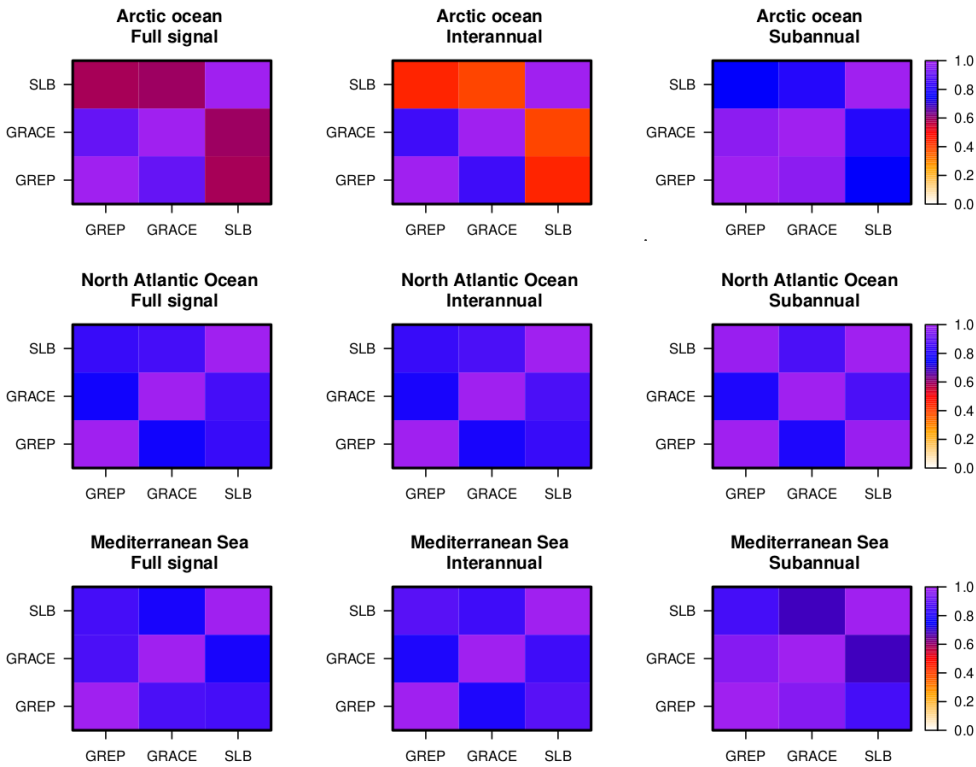
590 Figure 2. Correlation matrix for the three datasets in the three ocean basins investigated in this study, for both the full, the interannual, and the subannual signal. All values of correlation are statistically significant, at the 99% confidence level. Note the correlation matrix is symmetric, but all terms are shown in any case for the sake of clarity.
