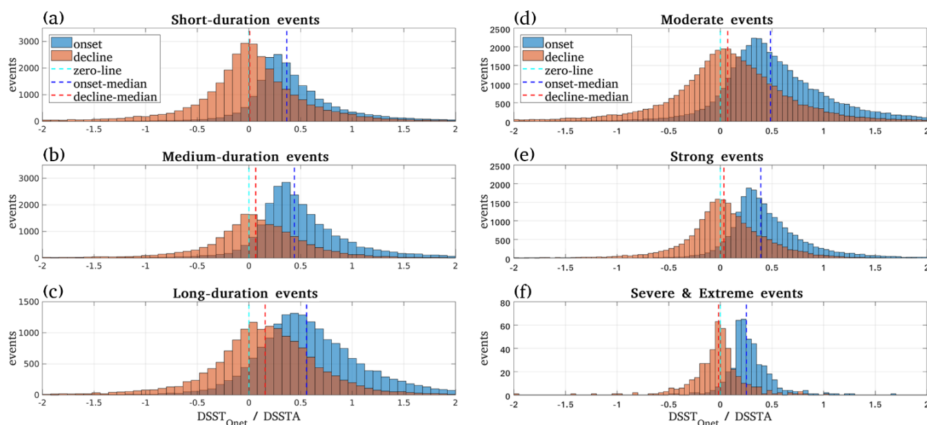
Figure 4 Left: Contribution of heat fluxes to the observed change in SSTA during MHW onset and decline phases, for the period 1993-2022, for phases lasting: less than 5 days (a), between 5-10 days (b) and more than 10 days (c) (short, medium and long duration phases, respectively). Right: Same as left but for different MHW severity categories: moderate (d), strong (e) and severe/extreme (f), based on the categorization scheme by Hobday et al. (2018).
