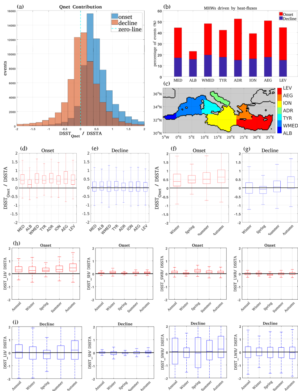
Figure 2 a) Contribution of heat fluxes to the observed change in SSTA during MHW onset and decline phases, for the period 1993-2022; b) Percentage of events primarily driven by heat fluxes (i.e., with more than half of the observed warming (cooling) attributed to heat fluxes during onset (decline)) for the entire Mediterranean Sea and sub-regions mapped in (c); d-e) Boxplots for the contribution of heat fluxes during onset (red) and decline (blue) for the entire Mediterranean Sea and the sub-regions; f-g) Boxplots for heat flux contribution per season, for onset (red) and decline (blue); h-i) Boxplots per season, for the contribution of heat flux components during onset (red) and decline (blue); From left to right: Latent heat flux, sensible heat flux, net short-wave radiation, net long-wave radiation. Notes: Positive heat-flux contribution during onset (decline) means that heat-fluxes warm (cool) the sea surface; boxes in boxplots define the interquartile range from the 25 th up to the 75 th percentile and whisker bars correspond to values falling within 1.5 times the interquartile range.
