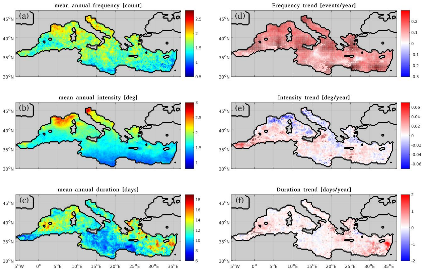
Figure 1 Left: Mean annual frequency, intensity and duration of MHWs for the period 1993-2022 (a, b, c, respectively); Right: Linear trends of annual values of frequency, intensity and duration (d, e, f, respectively). Black dots superimposed on trend fields correspond to statistically significant trends (Mann Kendall test, 95% confidence level)
