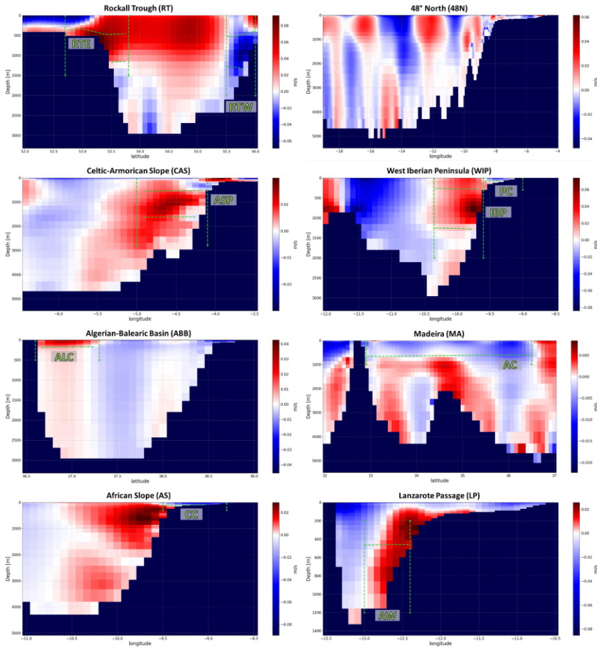
Figure 2: Mean vertical sections of transverse velocity along the transects defined in Figure 1 computed from IBI-REA over the period 1993-2021. Green dashed lines correspond to the monitoring windows defined to describe the variability of the currents defined. RTW: Rockall Trough Westward, RTE: Rockall Trough Eastward, ASP: Armorian Slope Poleward, IBP: Iberian Poleward, PC: Portugal Current, ALC: Algerian Current, CC: Canary Current, AC: Azores Current and AW: Antarctic Water.
