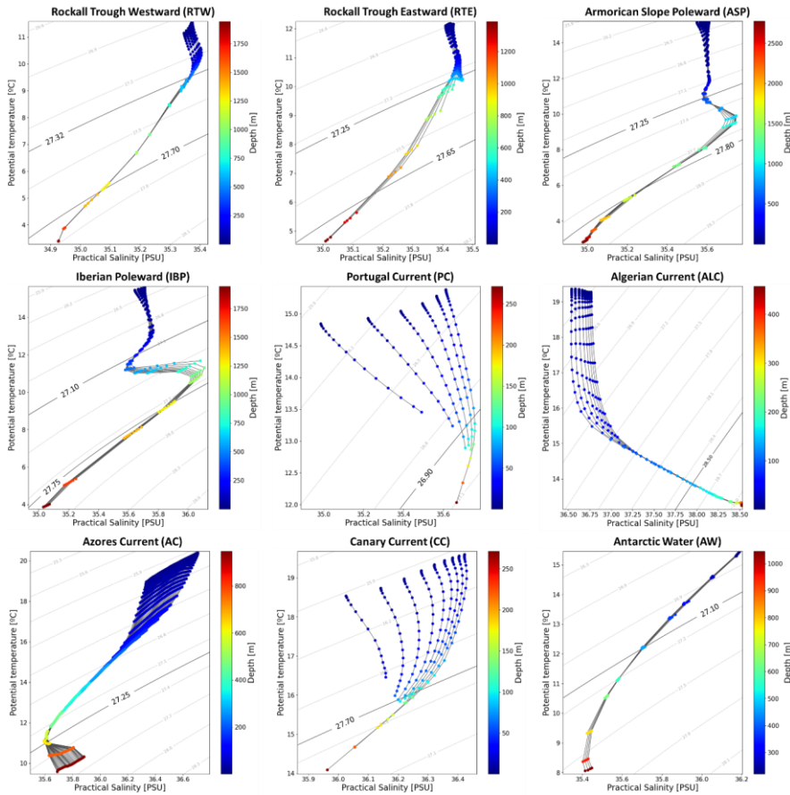
Figure 3: Averaged \theta/\sigma diagrams computed on the monitoring sections using IBI-MY product data over the period 1993-2021. Traces correspond to each vertical profile included on the corresponding monitoring window. The diagrams include the anomaly of potential density field (shown as dotted grey lines), being the vertical boundaries of each monitoring section represented by the black continuous lines. The diagrams that have a single continuous line correspond to monitoring windows where one of their vertical levels is defined as surface or seafloor (see Table 2).
