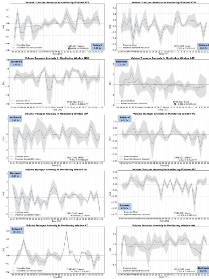
500 Figure 4: Annual anomalies of cross-section volume transport averaged in monitoring windows RTE, RTW, N48, ASP, IBP, PC, AC, ALC, CC, and AW. Time series computed and averaged from different Copernicus Marine products for each window (see Table 2) providing a multi-product result. The blue line represents the ensemble mean, and shaded grey areas represent the standard deviation of the ensemble. Blue boxes include the direction of the current and mean transport computed in the period 1993-2021. Red dashed lines depict the velocity value at which the direction of the current reverses. This aligns with the average transport value (with sign reversed) and the point where absolute transport becomes zero. The analysis of trends (at 95% confidence interval) computed in the period 1993–2021 is included (bottom right box). Trend lines (gray dashed line) are only 505
