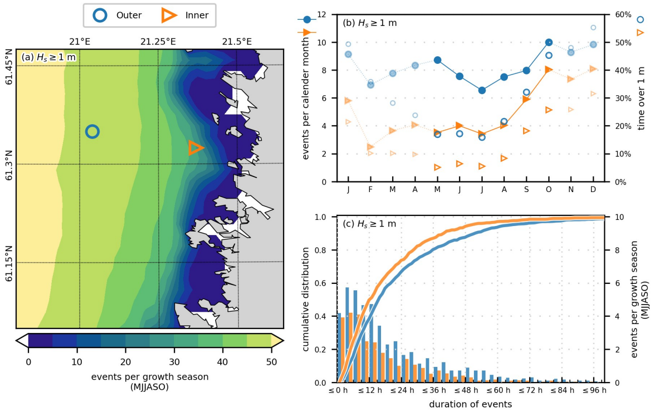
135 Figure 3: Events when the significant wave height ( H_s ) exceeded 1 m during the growth season of Rainbow trout in Finland (May to October). Number of exceedances per growth season (a), event occurrence from two locations as function of calendar month (b, left axis, filled symbols) and percentage of time H_s stayed over 1 m (b, right axis, empty symbols). The duration of the events during the growth season is presented as solid lines and the number of each event length is indicated as histogram (c). Bin size of histogram is 3 h so that first blue and orange bar correspond to event durations of 1, 2 and 3 h. Symbols and colours in (b,c) 140 correspond to locations in (a).
