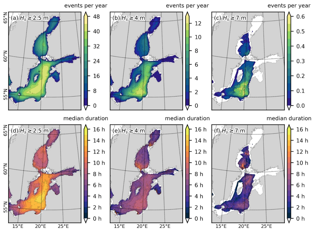
110 Figure 1: Number of events per year (a–c) and median duration in hours (d–f) of cases where H_s exceeds different thresholds: 2.5 m (a,d), 4 m (b,e) and 7 m (c,f). Values are calculated from 29 years hourly data from Baltic Sea wave hindcast (product ref. no. 1, Table 1).
