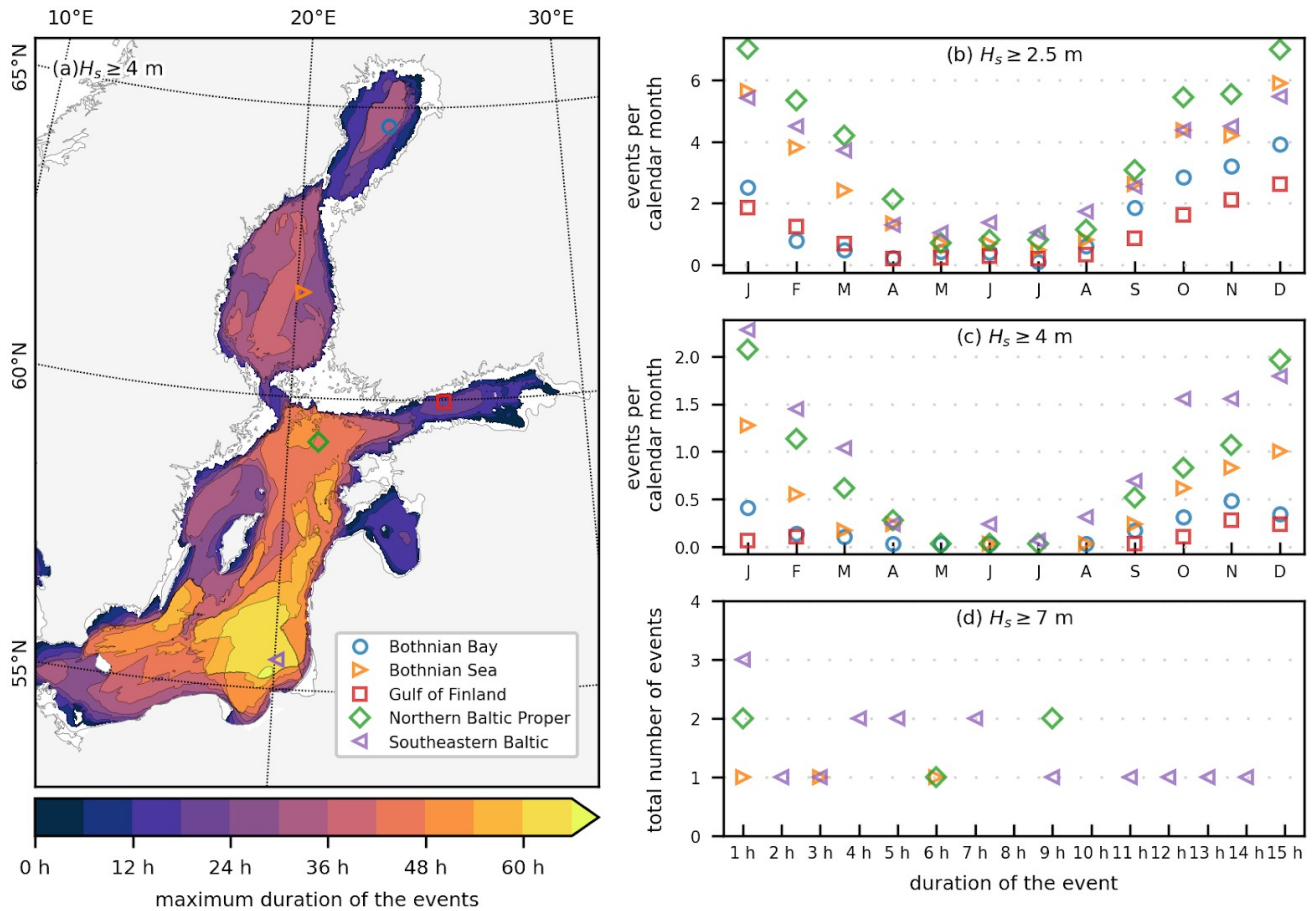
115 Figure 2: The maximum duration of events during 1993–2021 where the significant wave height exceeded 4 m (a). The event incidence for thresholds of 2.5 m and 4 m as a function of the calendar month (b&c). The number of events exceeding 7 m during the entire 29 year period as a function of the exceedance duration in hours (d). The symbols in b)–d) refer to the areas given in a).
