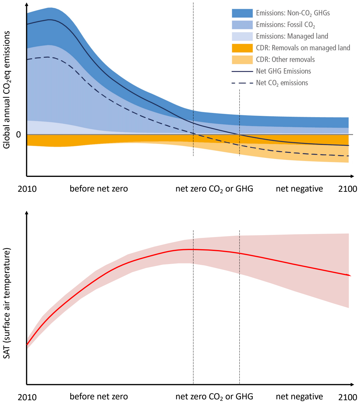
Figure 1: Top: The role of CO 2 removal (“CDR”) in a stylised pathway of ambitious climate. Dark orange illustrates CO 2 removals from land management and light orange illustrates removal from other CDR methods, including ocean-based methods. Note that net-zero CO 2 is reached well before net-zero greenhouse gas (GHG), and the amount of CDR required for net-zero CO 2 can be substantially smaller than the amount of CDR required for non-zero GHG. Any contribution of Ocean Alkalinity Enhancement
