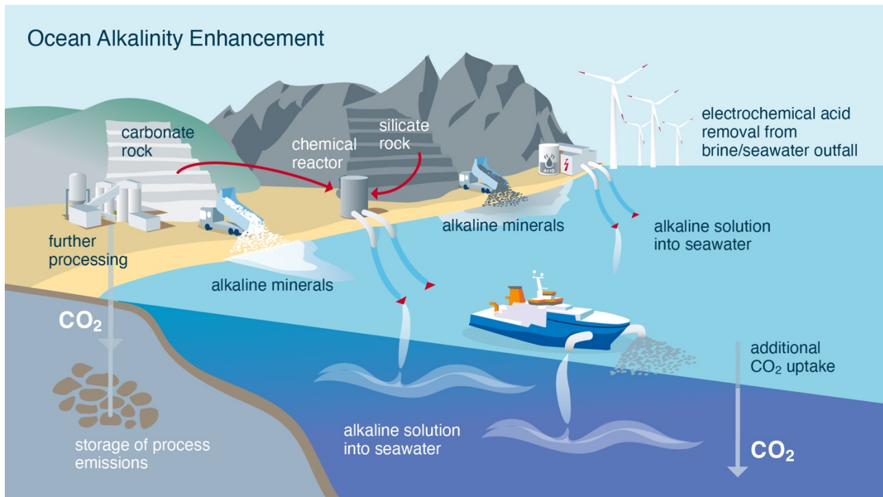
Figure 2: Illustration of various methods that have been proposed as Ocean Alkalinity Enhancement measure to achieve Carbon Dioxide Removal.
