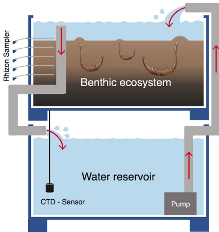
617 Figure 3: In the benthic mesocosms at the University of Antwerp the dissolution kinetics of silicate minerals and 618 the impacts on the benthic fauna in coastal environments are monitored since 2019. The system comprises 20 619 units with two stacked tanks, the upper tank is housing the benthic ecosystem, and the lower tank is functioning 620 as a water reservoir. Natural sediment of 40 sediment height with a mean grain size of 123 \mu\text{m} (3.0 phi) was 621 collected from an intertidal sand flat in the Oosterschelde (Netherlands) and mixed with olivine sand of similar 622 grain size. Water from the Easter Scheldt Estuary (salinity 32-35) is used to conduct flux-sessions of 5 weeks 623 (weekly sampling). At the end of each session, the total volume of water in each unit (~500 L) is renewed 624 (Drawing: A. Hylén, Photo: M. Kreuzburg https://www.coastal-carbon.eu/ , Geobiology, University of Antwerp).
