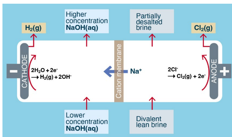
165 Figure 4. Typical process flow for the electrolytic conversion of aqueous \text{NaCl} -rich brine into alkalinity using the chlor-alkali membrane process. A chlor-alkali diaphragm process also exists but is not shown (Kumar, Du, and Lienhard, 2021).
