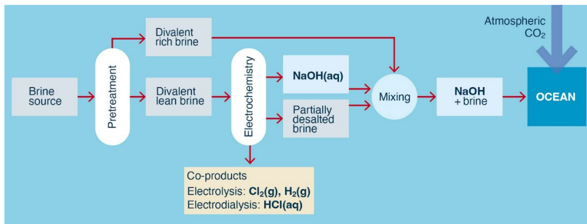
Figure 3. Process flow for the electrochemical conversion of aqueous chloride brine into alkalinity.
