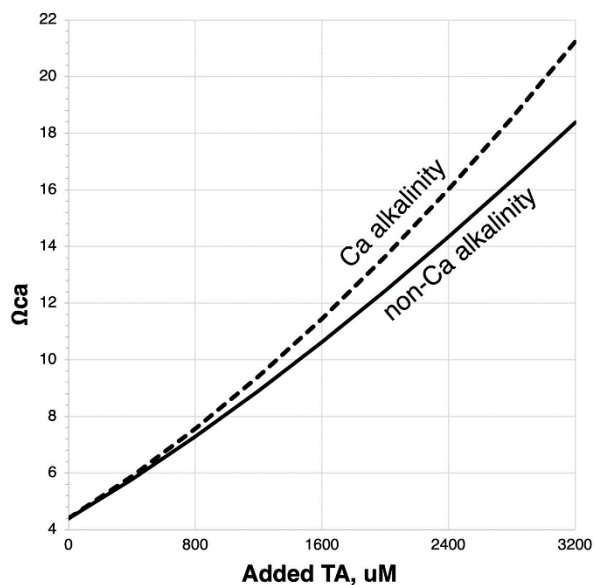
380 Figure 9. \Omega_{ca} (= the saturation state of calcite) response to calcium-based vs non-calcium-based alkalinity added to seawater initially containing 2350 \mu\text{M} total alkalinity (=TA) and equilibrated with a p\text{CO}_2 of 420 \mu\text{atms} . Modelled using \text{CO}_2\text{SYS} (Pierrot 2006) modified to account for variable [\text{Ca}^{2+}] .
