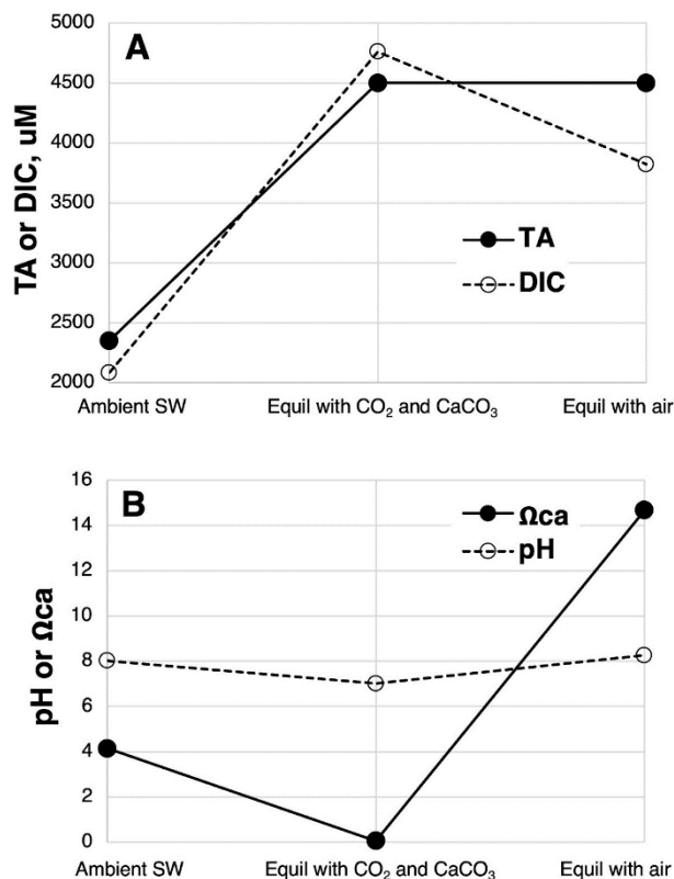
Figure 10. Example of the chemical progression of AWL starting first with representative, ambient seawater at p\text{ CO}_2=420\ \mu\text{atms} , followed by equilibration with \text{CaCO}_3 and a p\text{ CO}_2 of 10,000\ \mu\text{atms} followed by re-equilibration with air p\text{ CO}_2=420\ \mu\text{atms} . A) DIC = total dissolved inorganic carbon; TA = total alkalinity. B) \Omega_{ca} = the saturation state of calcite. Modelled using \text{CO}_2\text{SYS} (Pierrot 2006) modified to account for variable [\text{Ca}^{2+}] .
