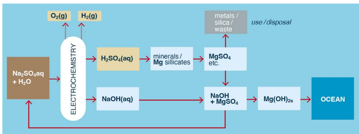
Figure 7. Example of the indirect production of solid, polyvalent metal hydroxides from minerals and water using electroanalysis or electrolysis of a monovalent salt. \text{H}_2 and \text{O}_2 are also produced.
