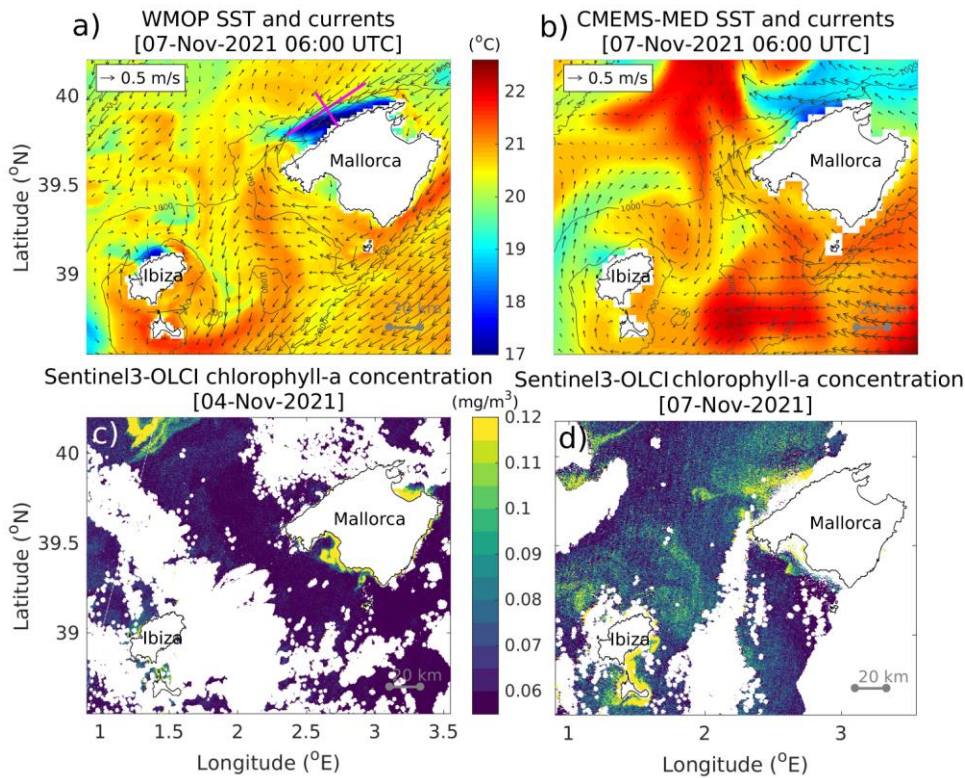
Figure 2: Upper panels: SST and surface currents around Mallorca and Ibiza Islands on 7 November 2021 at 06:00 UTC as represented by a) WMOP and b) CMEMS-MED models. In panel a), the lines in magenta represent the alongshore and cross-shore sections used in Sections 3 and 4. Lower panels: chlorophyll-a concentration as observed by Sentinel3-OLCI on c) 4 November and d) 7 November (i.e. before and during storm Blas, respectively).
