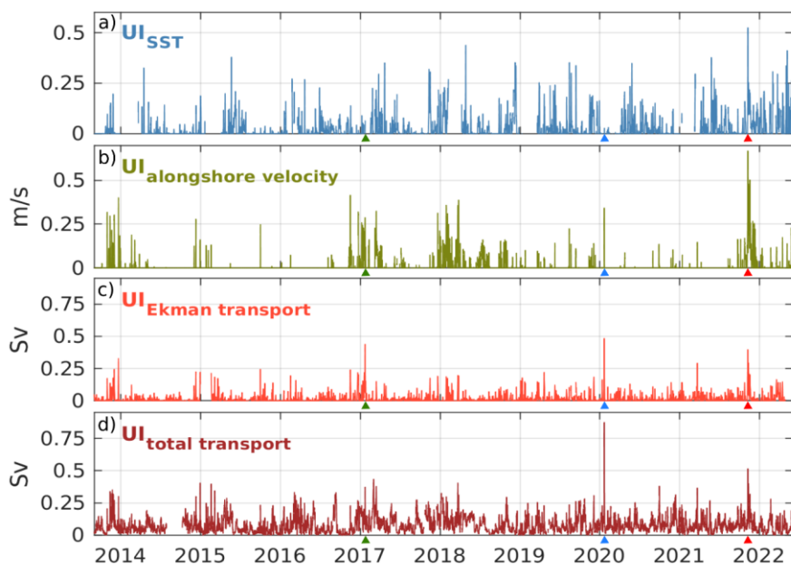
Figure 4: Time series of daily-upwelling indices defined in Section 2.3 between August 2013 and June 2022 ( 3-hourly values are shown after applying a 24-hour running average ): a) cross-shore normalized SST gradient index, b) alongshore velocity index, c) cross-shore Ekman transport index, d) cross-shore total transport index. The red, blue and green triangles on the x-axis mark the time of Blas, Gloria and January 2017 storms, respectively.
