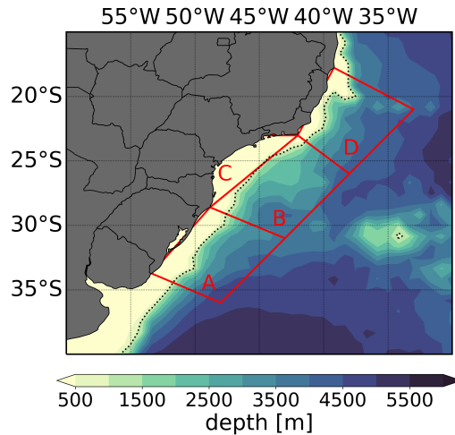
Figure 1. The Southwestern South Atlantic Ocean with the A to D subareas defined by the Brazilian Navy for warning and monitoring operations within MetArea V. Shaded values are the bathymetry from ETOPO1.
