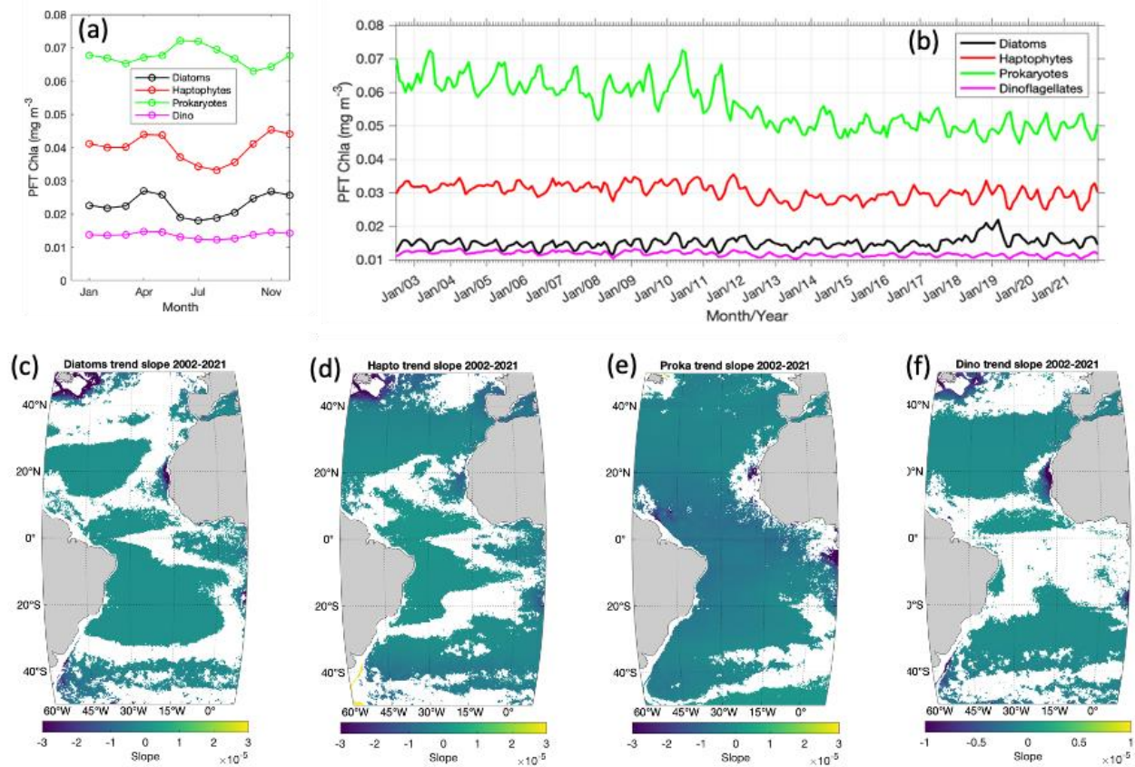
515 Figure 3: (a) Annual cycle of the four PFTs of diatoms, haptophytes, prokaryotes and dinoflagellates in the Atlantic Ocean (-50°S to 50°N, 60°W to 10°E), (b) 20-year time series from 2002 to 2021, and (c) per-pixel slope based on monthly Chla products of diatoms, (d) haptophytes, (e) prokaryotes and (f) dinoflagellates from 2002 to 2021 (where p < 0.05 were shown, slope unit: Chla mg m -3 month -1 ).
