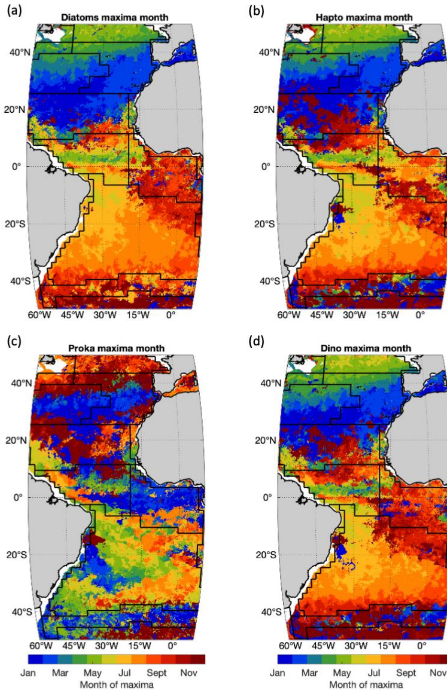
530 Figure 5: Occurrence month of PFT Chla maxima of 2021 in different provinces for (a) diatoms, (b) haptophytes, (c) prokaryotes and (d) dinoflagellates. Black lines indicate boundaries of Longhurst provinces as in Fig. 4.
