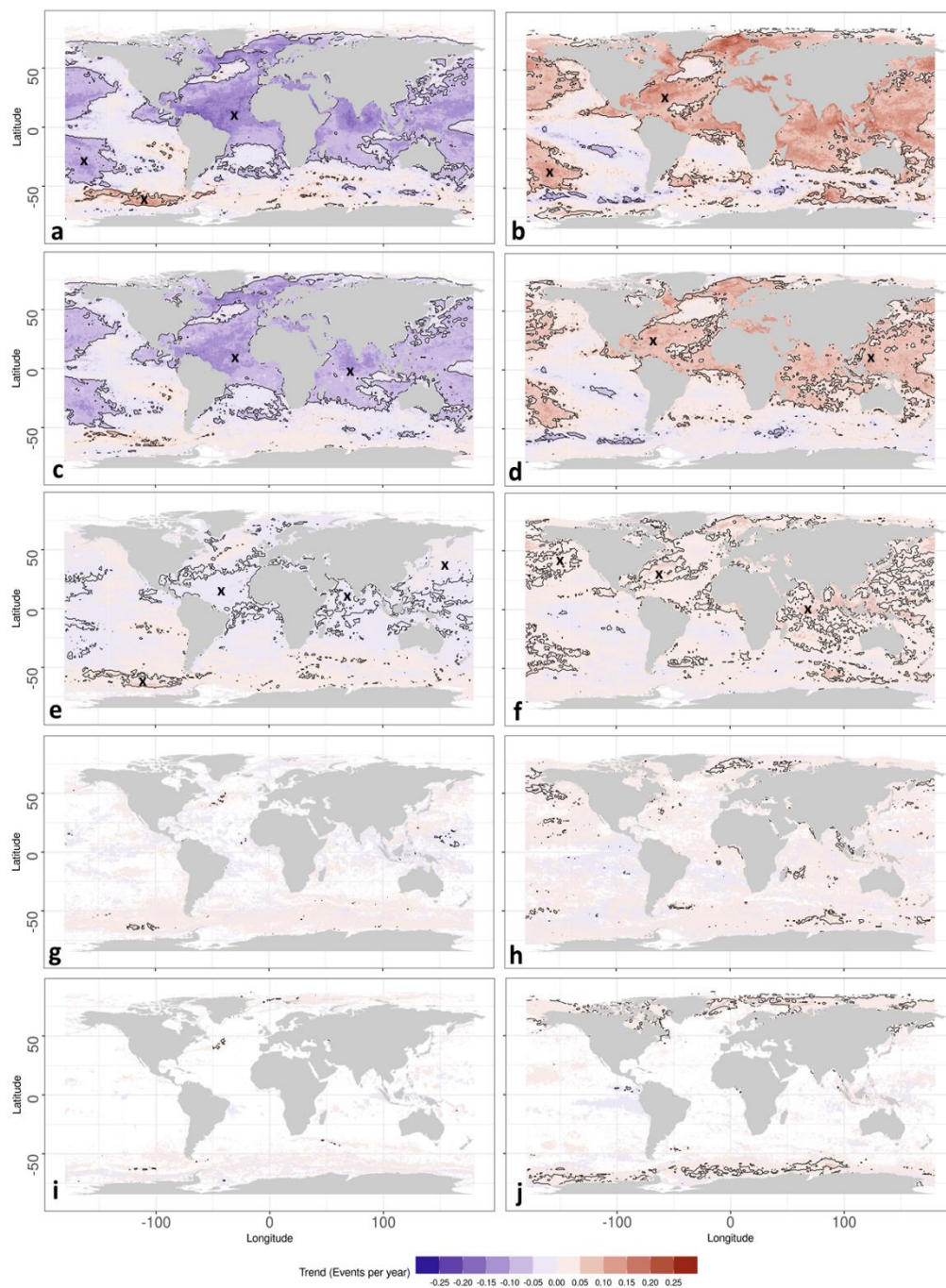
355 Figure 3: Trends in the number of MCS and MHW events per year for a) All MCS b) All MHW c), e), g), i) Category I-IV MCS d), f), h), j) Category I-IV MHW. The year of an event has been defined as the year of peak intensity. Linear trends were calculated using least squares fit, and the contour line bounds the region where the trends exceed the 99% confidence level of a two-tailed t-test compared to a constant rate of occurrence. The X markers indicate the inside of the contour to aid interpretation. Areas with no shading are where no events were detected.
