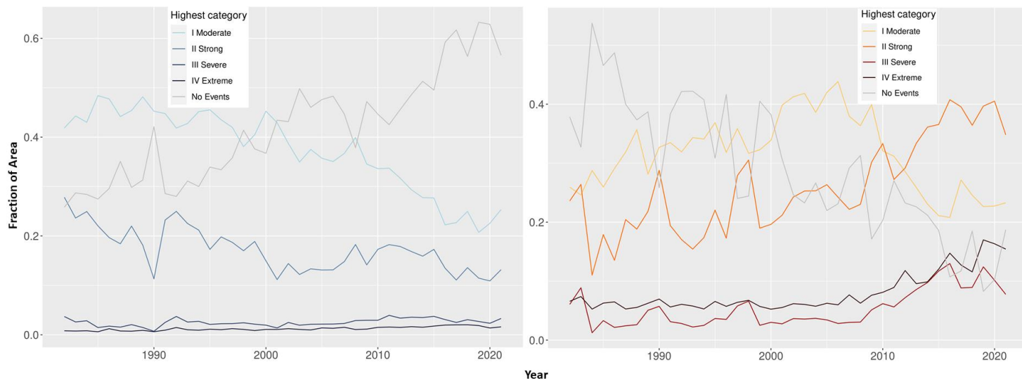
360 Figure 4: The fraction of the area of the ocean where the highest MCS (left) and MHW (right) category detected was I, II, III, IV, or no events being detected. The year of an event is defined as the year of the peak intensity.
