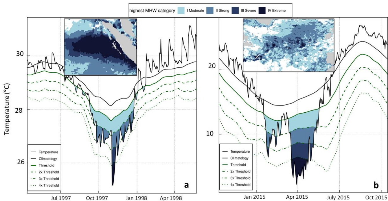
Figure 1: Significant MCSs. a) Sumatra 1997. Main figure: SST values and MCS threshold during late 1997 at the grid point 98.625, 0.875. Inset: Highest MCS category detected across the region during 1997 (the white cross denotes the location where the timeseries data was extracted). b) North Atlantic 2015. Main figure: SST values and MCS threshold during early 2015 at the grid point -50.375, 41.125. Inset: Highest MCS category detected across the region during 2015 (the white cross denotes the location where the timeseries data was extracted).
