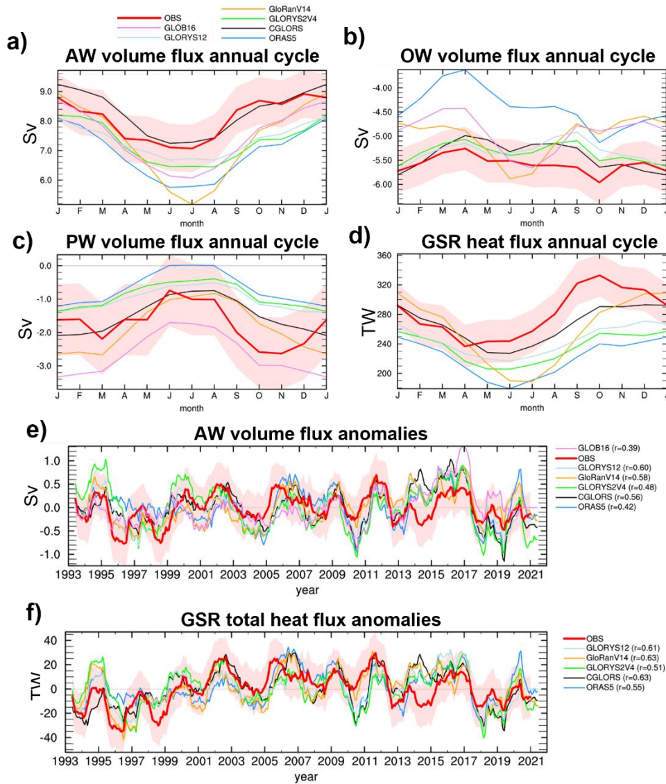
420 Fig. 2. Mean annual cycle of (a) AW volume flux (b), OW volume flux, (c) PW volume flux, and (d) GSR total (AW+PW+OW) heat flux; Temporal anomalies of (e) AW volume flux and (f) GSR total heat flux. The red shading indicates \pm 1 standard error of the observational data. Temporal correlations of reanalyses with observations are provided in the legends.
