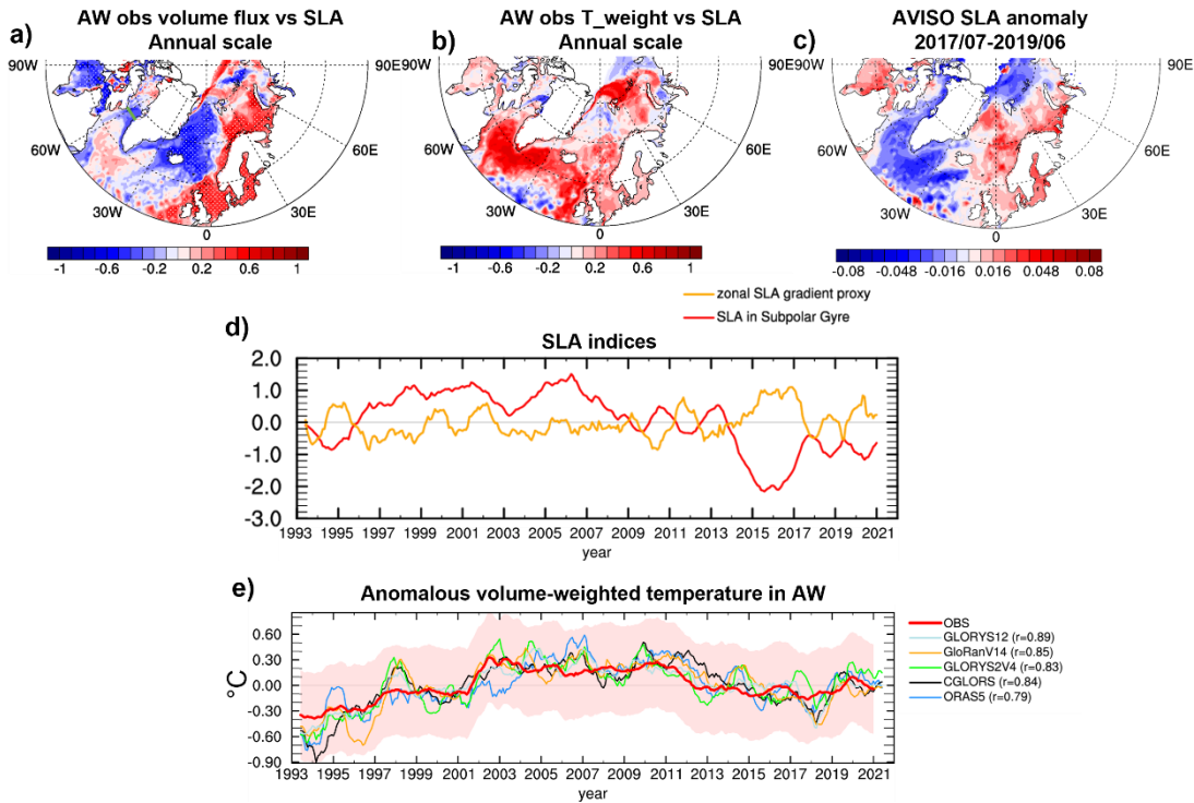
440 Fig. 4. Correlation of observation-based a) AW volume flux and b) AW flux-weighted temperature with SLA with a 12-monthly smoother applied; c) SLA anomaly in 2017/07-2019/06; d) temporal evolution (standardized) of two SLA-based indices based on the zonal SLA gradient at GSR and the SLA in the SPG region; e) temporal evolution of volume-weighted temperature anomalies of Atlantic waters at the GSR (red shading indicates \pm 1 standard error of the observational data and temporal correlations of reanalyses with observations are provided in the legend). Stippling in a) and b) denotes statistically significant correlations on the 95% confidence level.
