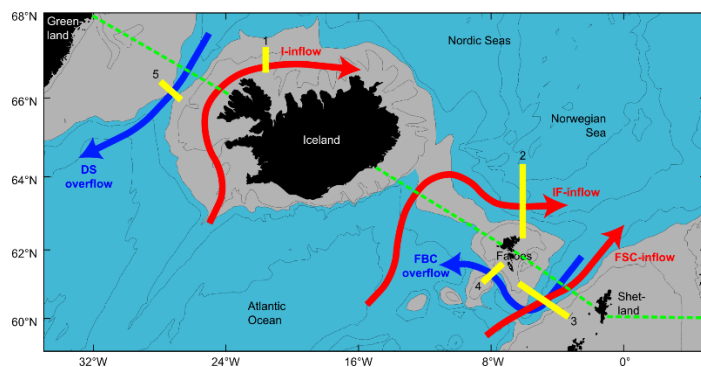
415 Fig. 1. Map of the Greenland-Scotland Ridge region, schematically depicting shallow shelf and deep water, major AW inflow (red arrows) and OW outflow (blue arrows) branches, location of oceanic moorings used for deriving the observation-based transport estimates (yellow bars), and the section used for computation of transports from ocean reanalyses (dashed green line). Adapted from OceanSITES ( http://www.oceansites.org/tma/gsr.html , Fig. 1).
