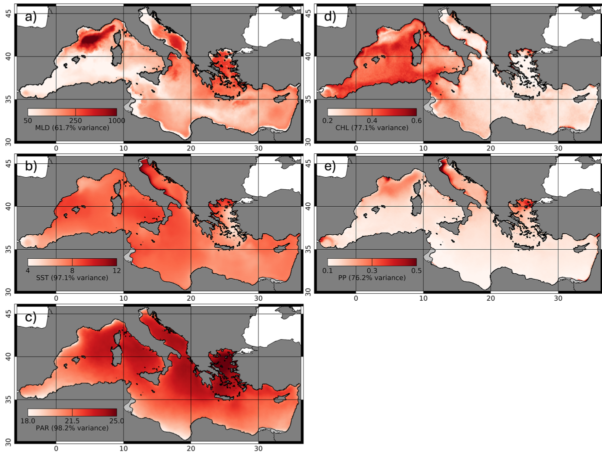
Figure 3. Spatial patterns of the first mode of EOF for MLD (a), SST (b), PAR (c), CHL (d), and PP (e). Light grey indicates the areas permanently masked out because of persistent or recurrent Case II water conditions.
