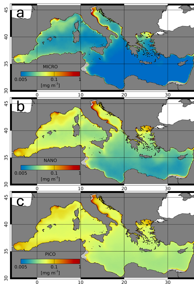
Figure B2. Mean time averages (1998–2025) of Microphytoplankton chlorophyll (a), Nanophytoplankton chlorophyll (b) and Pico-phytoplankton chlorophyll (c). Light grey indicates the areas permanently masked out because of persistent or recurrent Case II water conditions.
