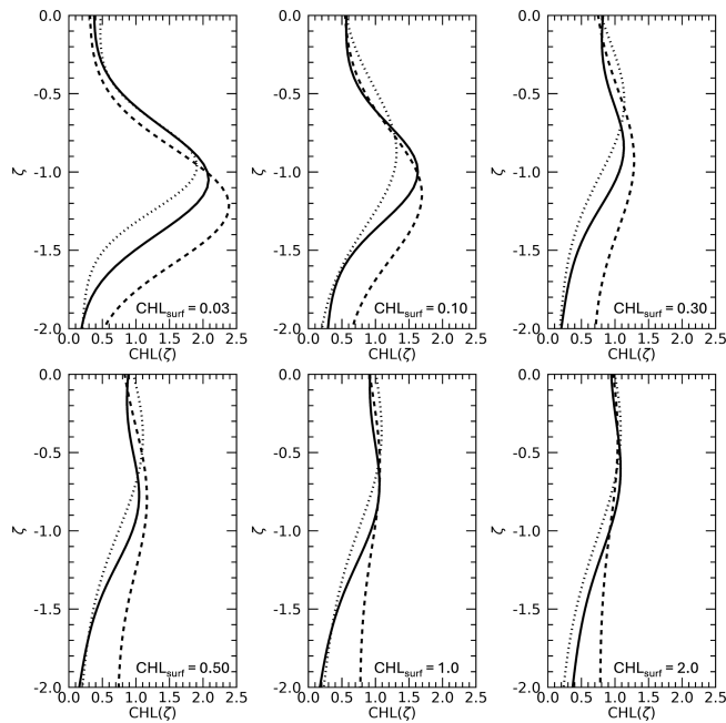
Figure A2. Reconstructed vertical chlorophyll profiles from the Mediterranean model (solid lines), Morel and Berthon (1989) (dashed lines) and Uitz et al. (2006) (dotted lines). The surface chlorophyll concentration (CHL surf ) is indicated in the bottom-right corner of each panel.
