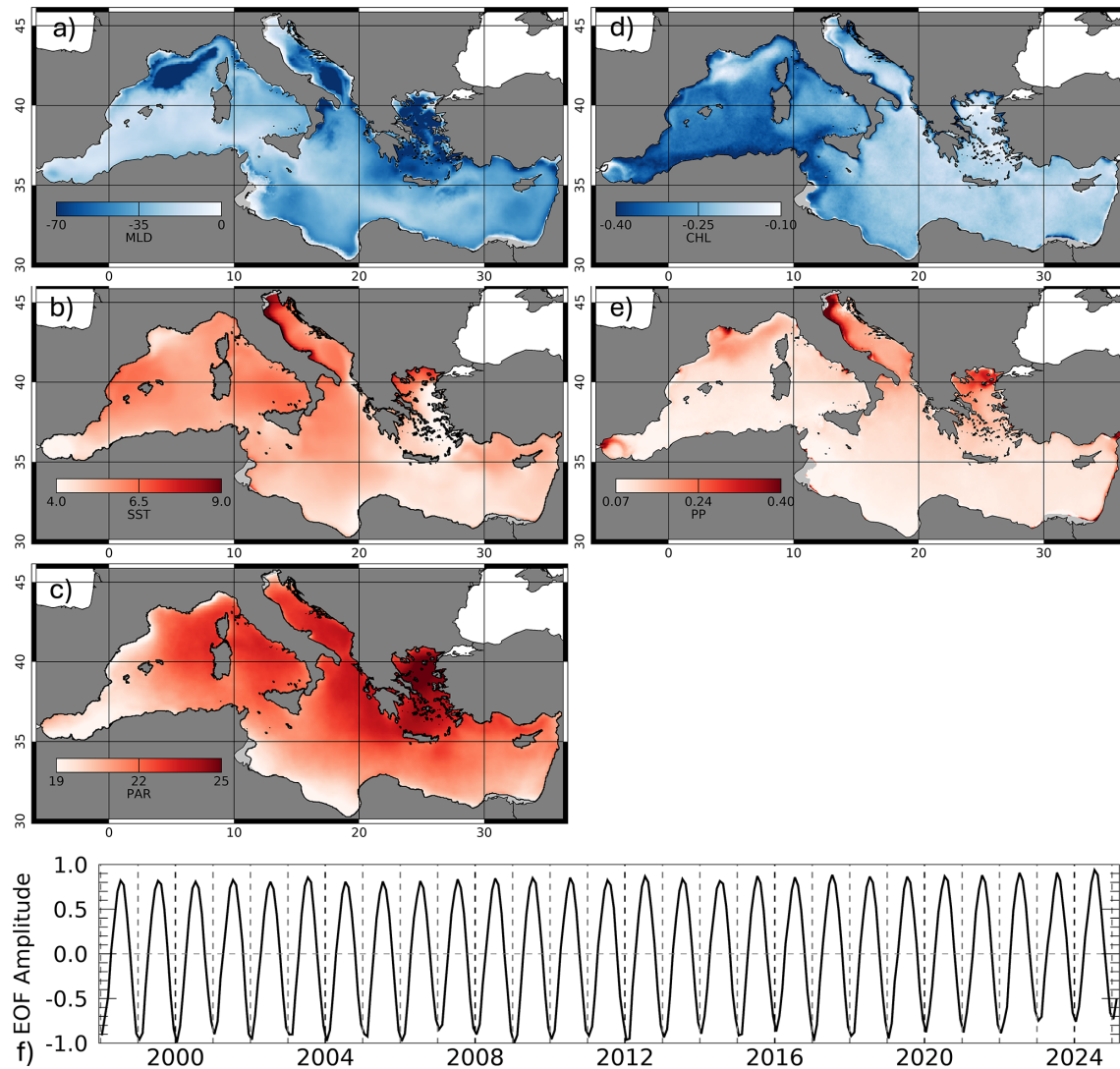
Figure 7. First mode of MEOF of MLD (a), SST (b), PAR (c), CHL (d) and PP (e) spatial patterns and temporal evolution (f). Light grey indicates the areas permanently masked out because of persistent or recurrent Case II water conditions.
