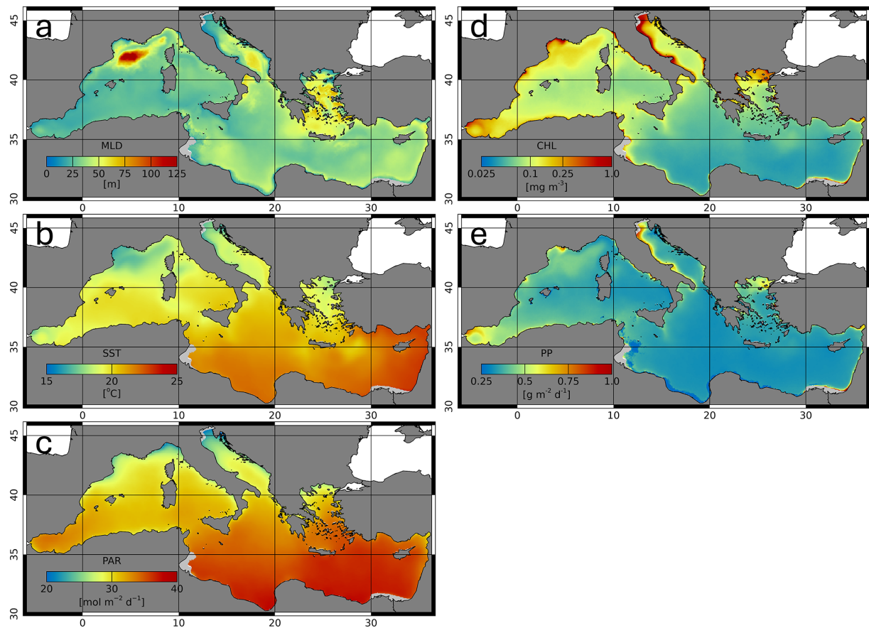
Figure 1. Mean time averages (1998–2025) of MLD (a), SST (b), PAR (c), CHL (d), and PP (e). Light grey indicates the areas permanently masked out because of persistent or recurrent Case II water conditions.
