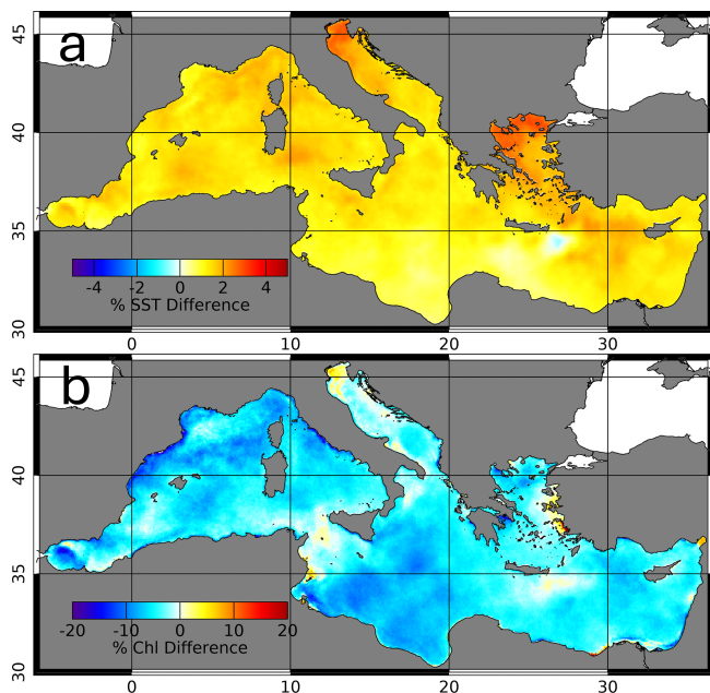
Figure B1. Relative percent difference RPD = 100 \frac{X-Y}{Y} , with Y being the mean time average (1998–2006) of SST and CHL for the same period as Volpe et al. (2012). X is the mean time average of SST (a) or CHL (b) computed over the full time range (1998–2025).
