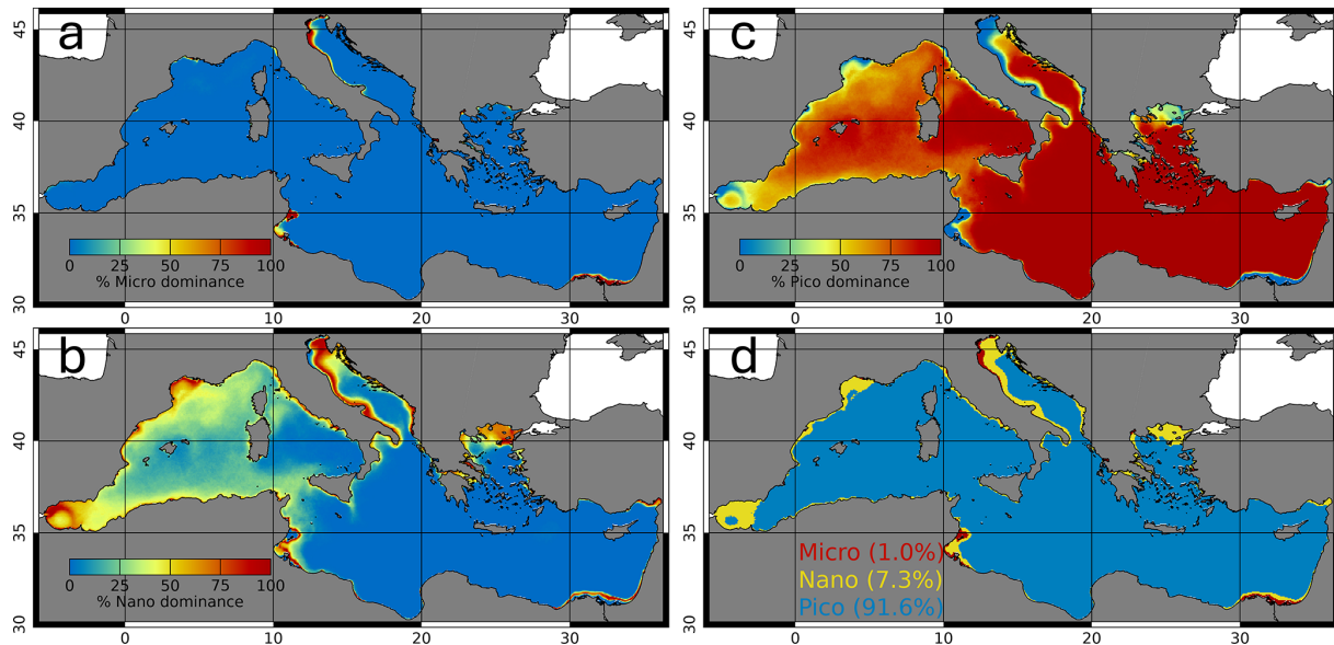
Figure 2. Percent dominance of PSC size classes (Micro, Nano and Pico in panels a , b and c , respectively) over time. Panel ( d ) shows the overall temporal dominance of each size class in percent over the entire time series.
