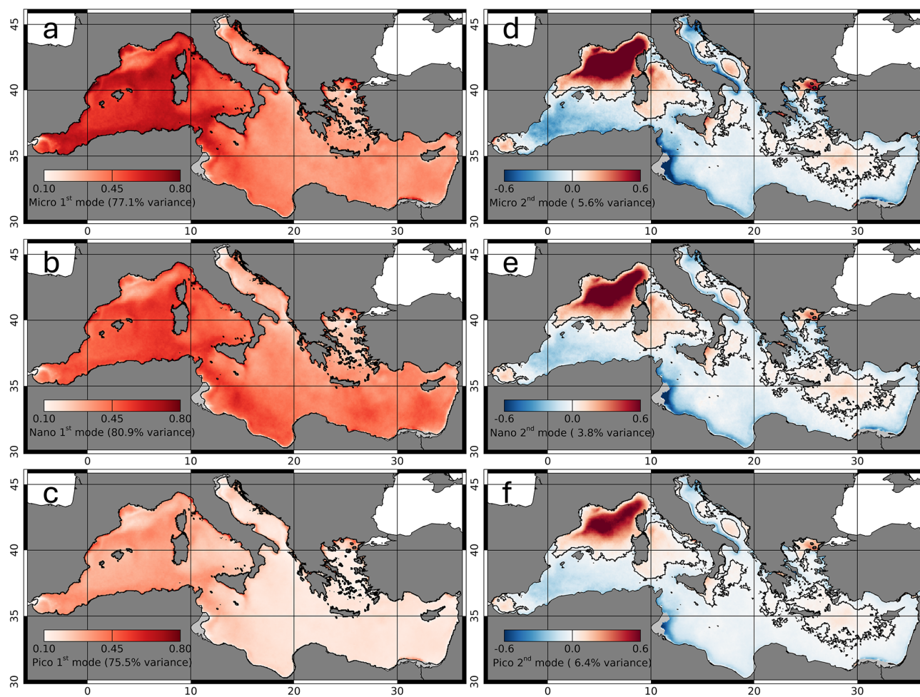
Figure B3. First two EOF spatial patterns computed over Micro- (a–d), Nano- (b–e) and Pico-phytoplankton (c–f). Light grey indicates the areas permanently masked out because of persistent or recurrent Case II water conditions.
