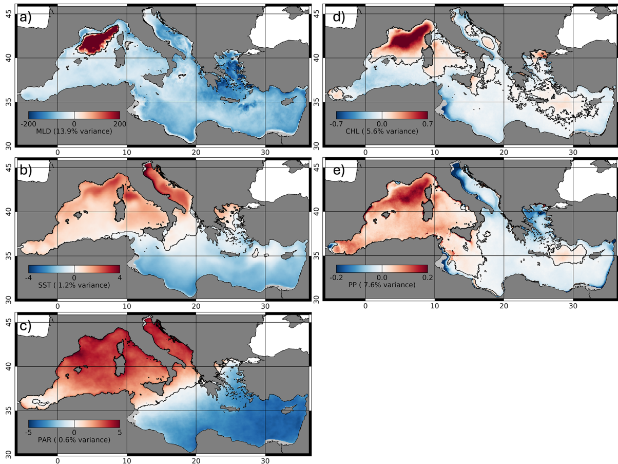
Figure 5. Second mode of EOF variability for MLD (a), SST (b), PAR (c), CHL (d) and PP (e) spatial patterns. Light grey indicates the areas permanently masked out because of persistent or recurrent Case II water conditions.
