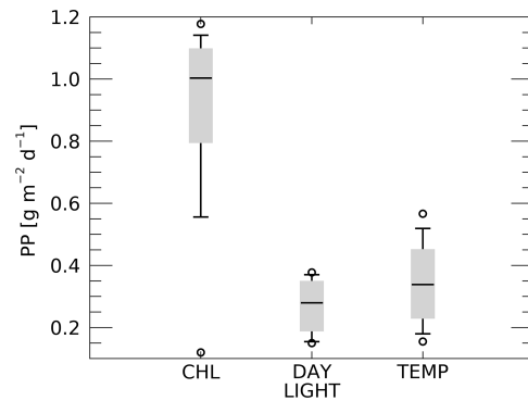
Figure A3. Sensitivity analysis of PP. The grey rectangles represent the interquartile range (25th–75th percentiles) of PP estimates obtained by varying each parameter individually. The horizontal line within each box marks the median (50th percentile). Whiskers denote the 10th and 90th percentiles, while circles indicate the minimum and maximum PP values. The abscissa indicates the input parameters analysed.
