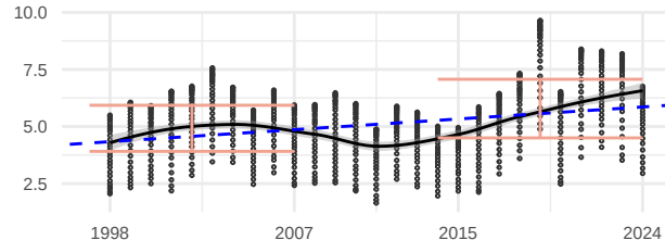
Bioregion 6; slope = 0.58%/decade; pvalue = 0.060
