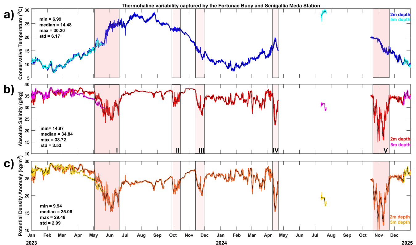
Figure 1. Hourly (colored lines) and daily-averaged (black dotted lines) time series of (a) conservative temperature, (b) absolute salinity, and (c) potential density anomaly recorded at 2 and 5 m depth offshore of Fano and Senigallia, respectively (product ref. 1 and 2; Table 1). Basic statistical descriptors (minimum, maximum, median, standard deviation) for each thermohaline property are reported in the top left corner of each panel. Light red shaded areas (I–V) indicate the timing of the five most significant surface freshening events identified between 2023 and 2024.
