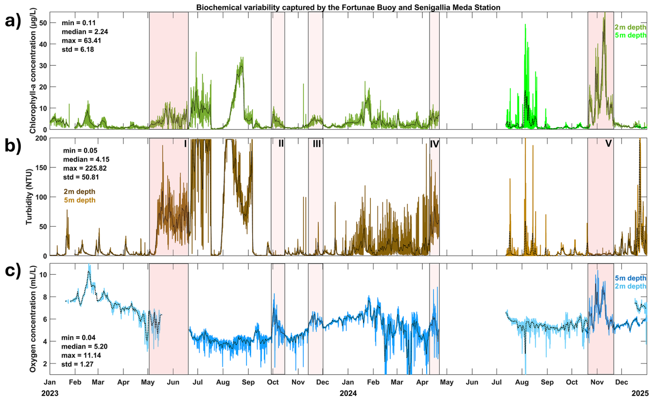
Figure 4. Hourly (colored lines) and daily-averaged (black dotted lines) time series of (a) chlorophyll a concentration, (b) turbidity, and (c) dissolved oxygen concentration measured at 2 and 5 m depths by the Fortunaie buoy (offshore of Fano) and the Senigallia Meda station, respectively (product ref. 1 and 2; Table 1). Basic statistical descriptors (minimum, maximum, median, standard deviation) are reported in the left corner of each panel. Red shaded areas (I–V) denote the timing of the five most pronounced surface freshening events as identified in Fig. 1. Biogeochemical responses, including sharp increases in turbidity and chlorophyll a , coincide with or follow these events, reflecting ecosystem perturbations.
