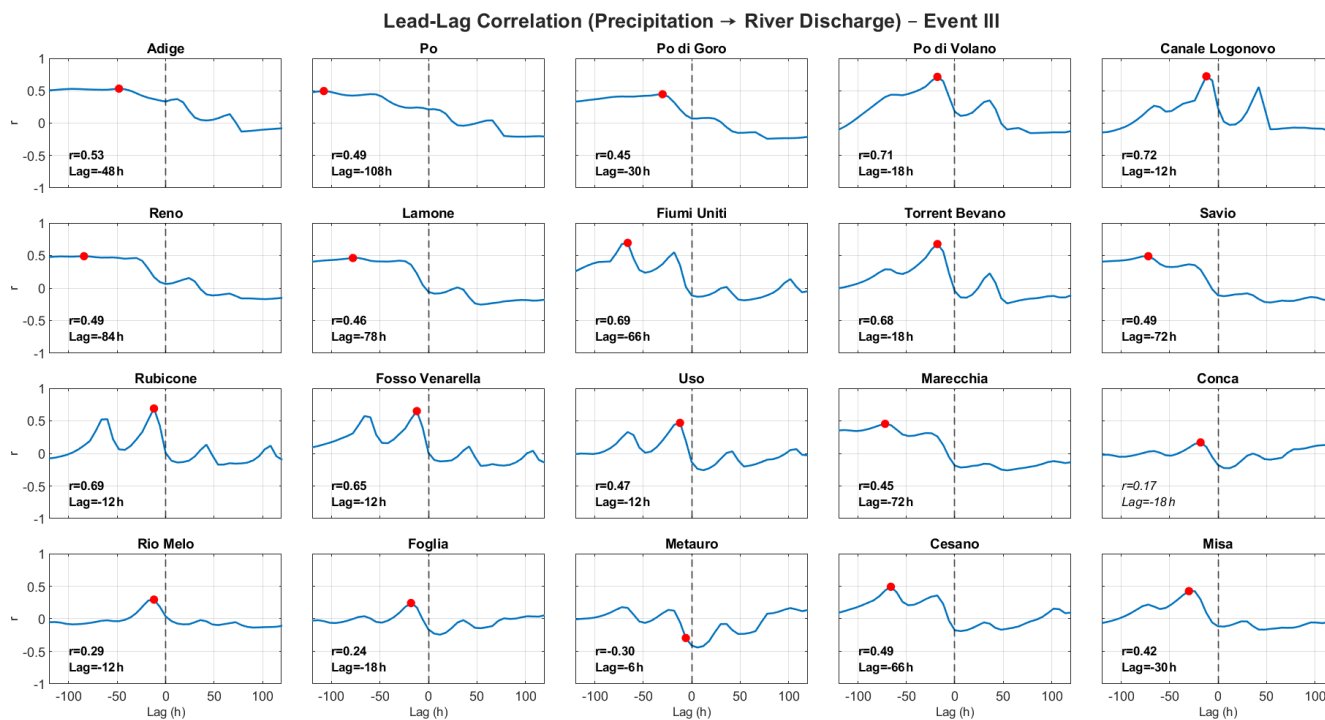
Figure A4. Same as Fig. A2 but for the third event.
