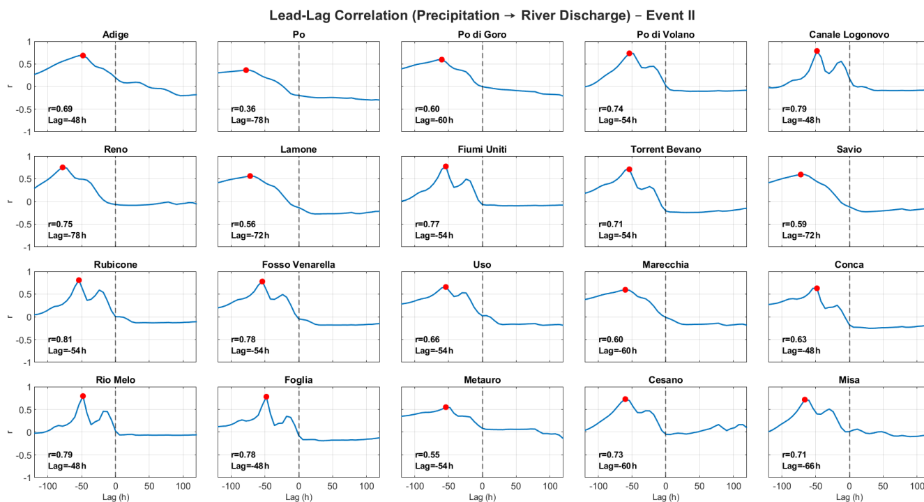
Figure A3. Same as Fig. A2 but for the second event.
