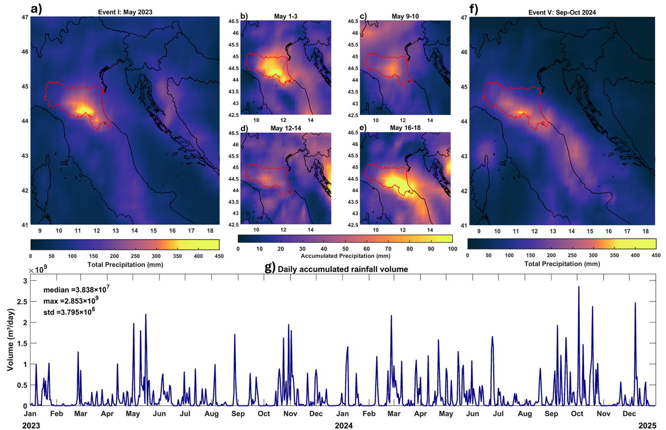
Figure 2. Spatial distribution of accumulated precipitation (product ref. 2; Table 1) over Emilia-Romagna and surrounding areas during key extreme rainfall events associated with surface freshening Event I and Event V (see Fig. 1). (a) Total precipitation during the combined May 2023 period (Event I). Accumulated precipitation during individual May 2023 storm episodes: (b) 1–3 May, (c) 9–10 May, (d) 12–14 May, and (e) 16–18 May. (f) Total precipitation during the two September–October 2024 events (Event V). The Emilia-Romagna region is outlined in red in each panel. (g) Time series of daily accumulated rainfall volume ( \text{m}^3 \text{d}^{-1} ) over the domain, highlighting the timing and intensity of individual rainfall peaks between January 2023 and December 2024. Basic statistical descriptors (minimum, maximum, median, standard deviation) are reported in the upper left corner.
