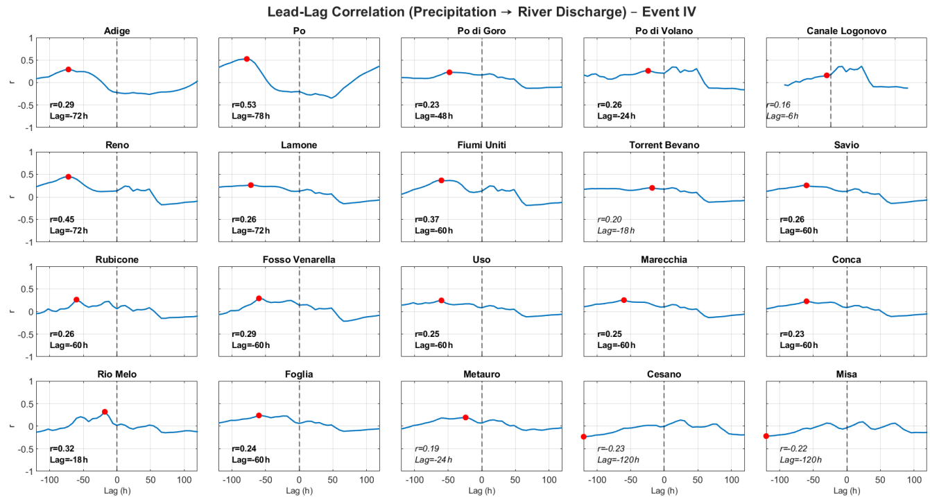
Figure A5. Same as Fig. A2 but for the fourth event.
