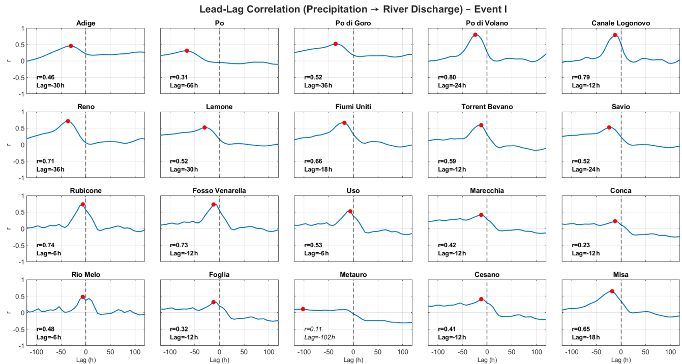
Figure A2. Lead-lag correlation plots between accumulated precipitation over the Emilia-Romagna region and the discharge of 20 rivers during the first major flooding periods that lead to the previously-defined freshening event I. Each subplot shows the Pearson correlation coefficient ( r ) as a function of lag time (in hours), where negative lags indicate that precipitation leads river discharge. The maximum correlation point for each river is marked with a red dot. Corresponding correlation values and lags are annotated in bold if statistically significant ( p < 0.05 ), and in italics otherwise.
