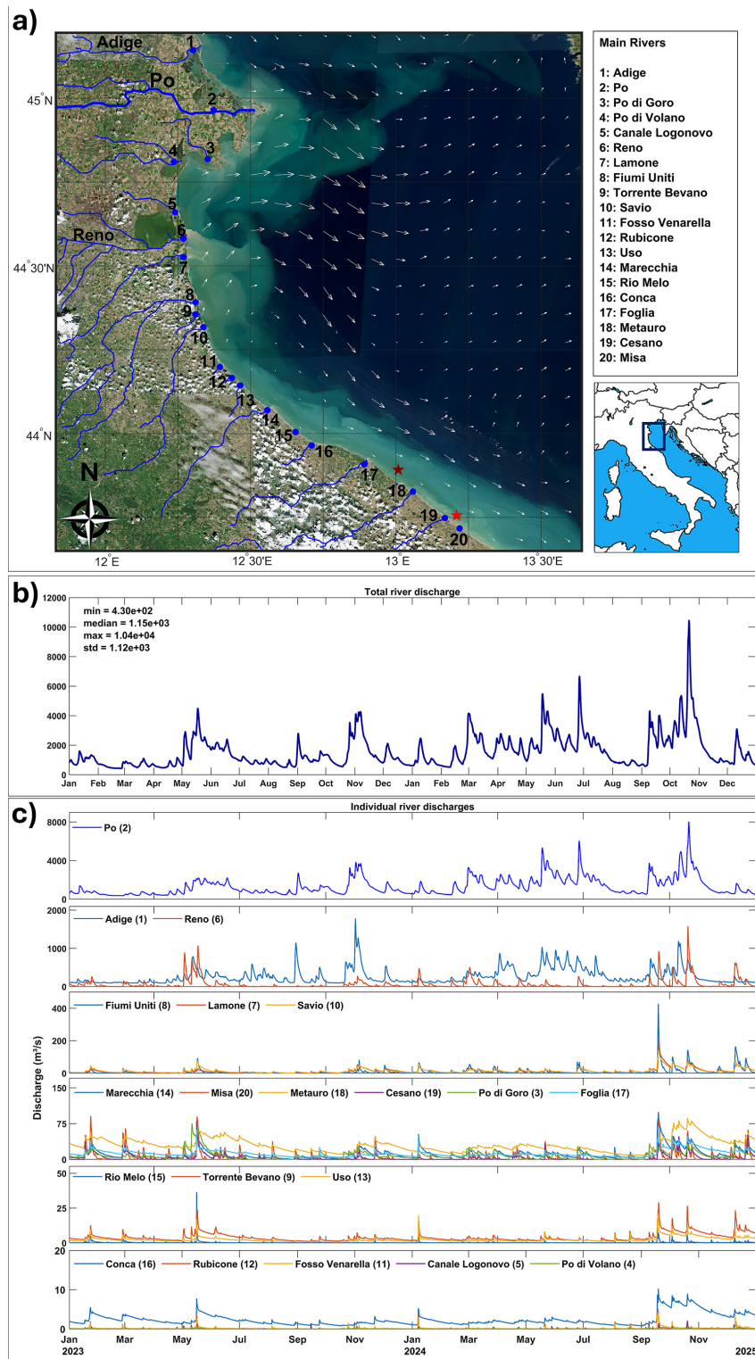
Figure 3. Overview of (a) the study area with the location of the 20 assessed river mouths (blue dots) and the positions of the autonomous monitoring platforms offshore of Fano and Senigallia (dark and light red star, respectively). The background corresponds to a Sentinel-2 Level 2A true-color image ( https://dataspace.copernicus.eu/browser , last access: 17 August 2025) acquired on 31 October 2024, overlaid with surface current vectors derived from the numerical circulation model (product ref. 8; Table 1) for the same date. (b) Daily time series of the total accumulated river discharge (m 3 s -1 ) from all 20 rivers for the period January 2023–December 2024 (product ref.3; Table 1). Key descriptive statistics (minimum, median, maximum, standard deviation) are indicated. (c) Individual river discharge time series, grouped by magnitude, with numeric labels corresponding to the river mouth positions indicated in panel (a).
