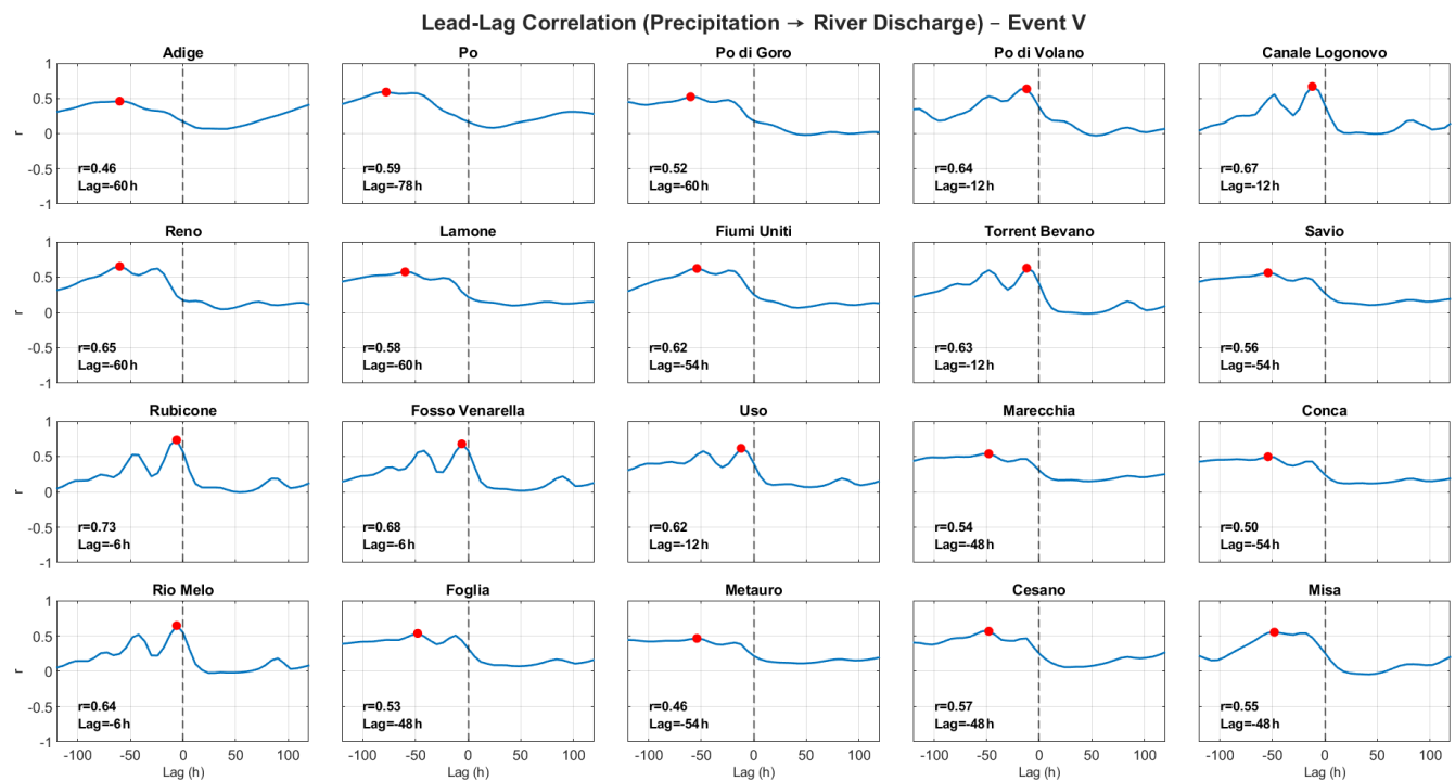
Figure A6. Same as Fig. A2 but for the fifth event.
