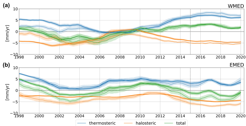
Figure 2. Time series of decadal trend associated to the de-seasoned total steric sea level ( \eta_S ), and its thermosteric ( \eta_T ) and halosteric ( \eta_H ) components, computed over sliding windows shifted by one month across the period 1993–2024 in the WMED (a) and EMED (b). Different datasets are shown: MEDREA24 (thick lines) and GLORYS12 (thin lines). Shaded areas represent the trend uncertainty, defined as the standard deviation of the residuals from the bootstrap procedure. The vertical dashed line at January 2015 marks the starting point of tide gauges analysis shown in Fig. 4.
