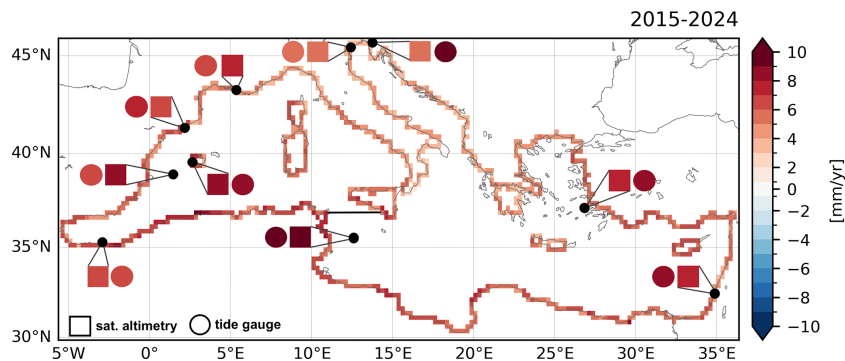
Figure 3. Map of decadal sea level trends computed at coastal points from the satC3S dataset for the 2015–2024 period. This decade is the most recent available for comparing decadal trends from satC3S altimetry (where DAC has been reintroduced), with in-situ observations from tgCMEMS and tgPSMSL, adjusted for VLM. Each black dot indicates the location of a tide gauge discussed in the text. Satellite and tide gauge-derived trends at the same sites are shown as squares and circles, respectively, and are coloured according to the colorbar (values reported in Table 3). The thin black line corresponds to the zonal transect used to define the boundary between WMED and EMED at 37° N.
