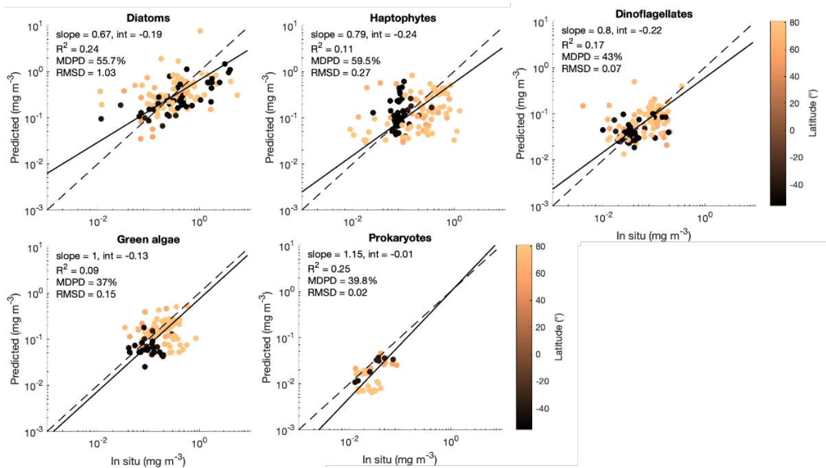
Figure S2. Original PFT Chla derived from OLCI sensors in comparison with in situ PFT dataset 2 (corresponding to Figure 3b, only own expeditions in high latitudes from 2021 to 2023, maximum number of points N=134 but varies for different PFTs due to possible absence).
