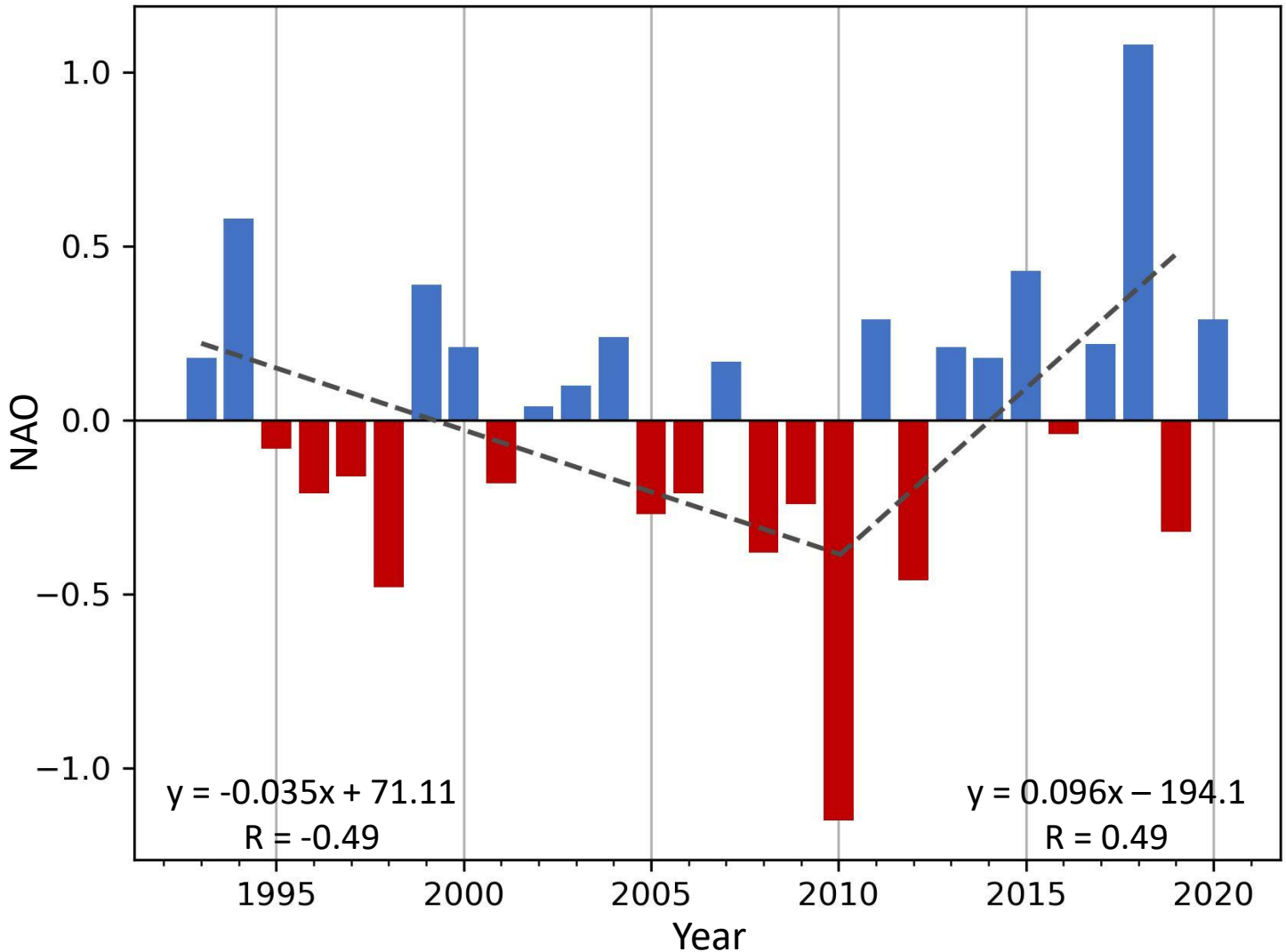
Figure S1: Annual average of North Atlantic Oscillation (NAO) index from 1993 to 2020. Dashed grey lines correspond to the trend line computed in the periods 1993-2010 and 2010-2019. The adjustment parameters for both periods are included at the bottom of the figure (left for period 1993-2010 and right for period 2010-2019).
