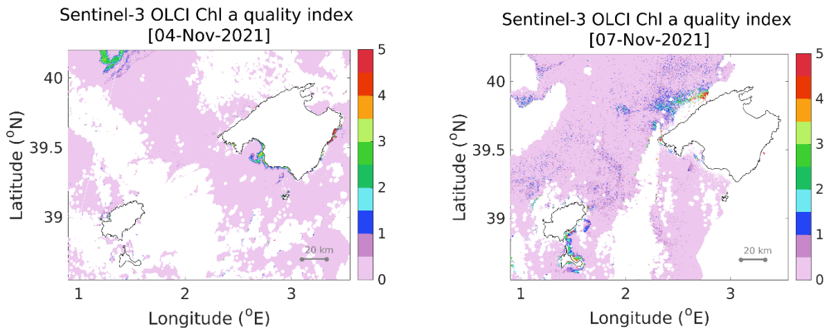
Figure S1: Quality Index (QI) of Sentinel-3 OLCI Chl a images on (left) 4 and (right) 7 November 2021
