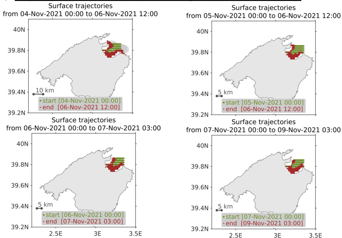
Figure S2: Surface trajectories of model particles seeded in Alcúdia Bay on 4 (top-left), 5 (top-right), 6 (bottom-left) and 7 (bottom-right) November at 00:00UTC. The initial and final positions are represented by green and red dots, respectively.
